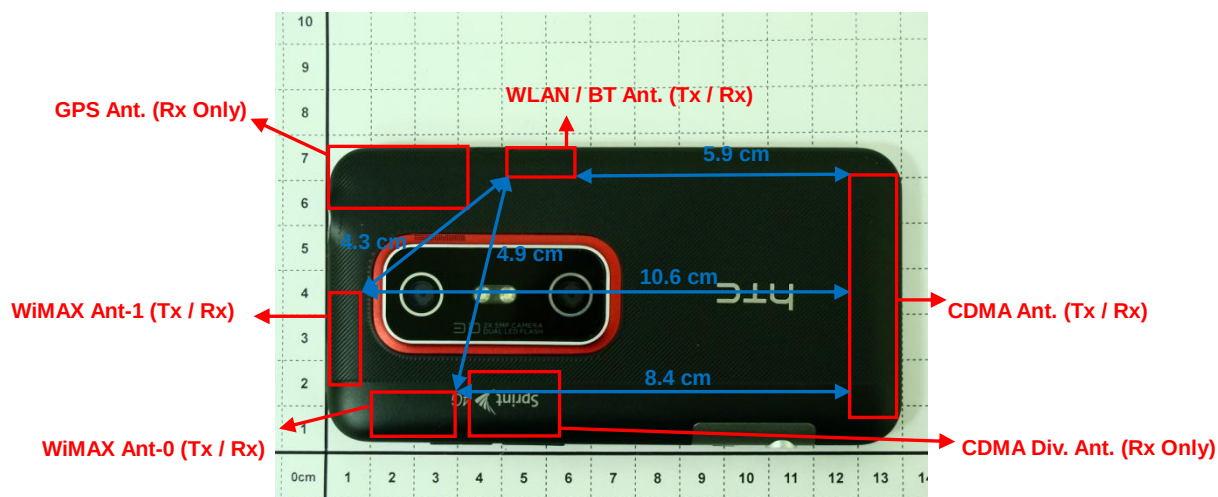
Antenna Location and Separation Distance
