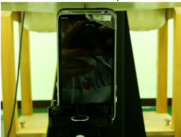
Top Side of the DUT with Phantom 1.0 cm Gap for DUT without Earphone
