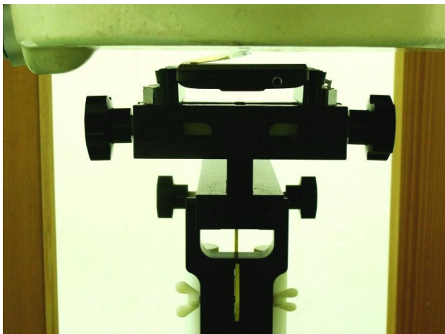
Front Face of the DUT with Phantom 1.0 cm Gap for DUT without Earphone
