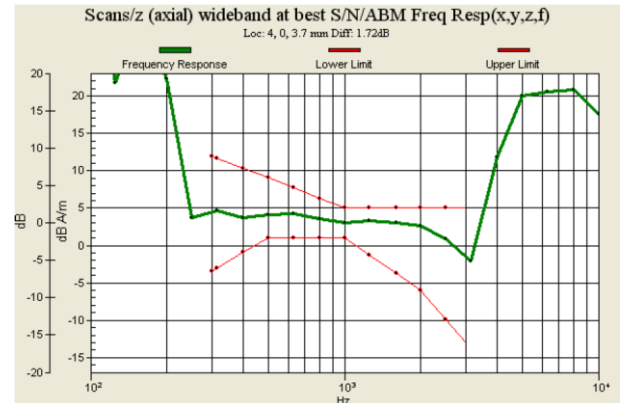
Fig. 9.8 CDMA2000 BC1 Ch1175 (DUT with Battery 2)
