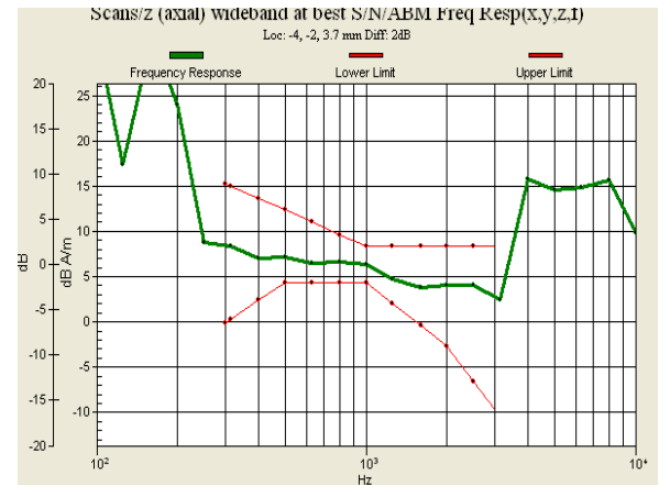
Fig. 9.4 CDMA2000 BC0 Ch1013 (DUT with Battery 2)
