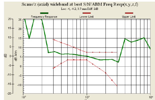
Fig. 9.6 CDMA2000 BC1 Ch600 (DUT with Battery 1)
