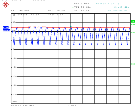
835MHz - 80% AM
