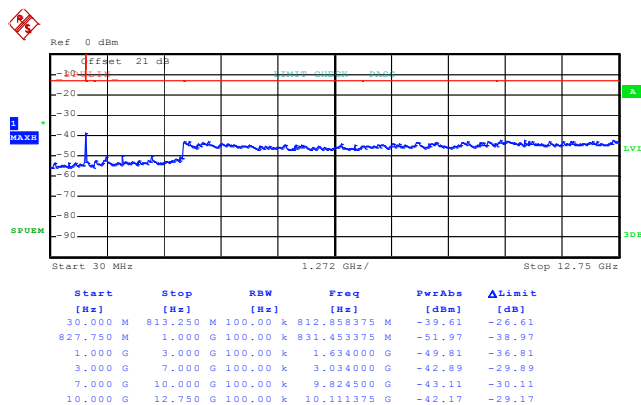
Conducted Emission Plot between on Channel 440
