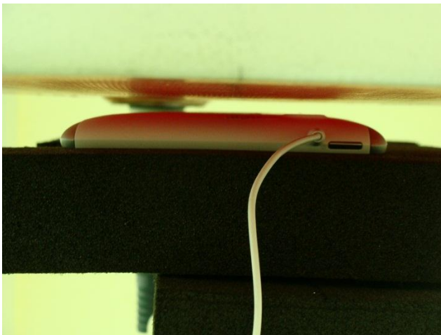
Rear Face of the DUT with Phantom 0.5 cm Gap
