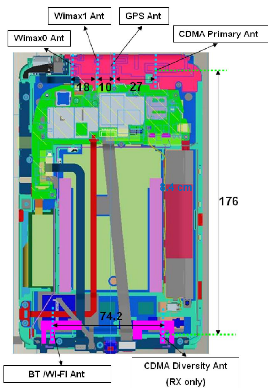
Antenna Location and Separation Distance (DUT Rear View)
