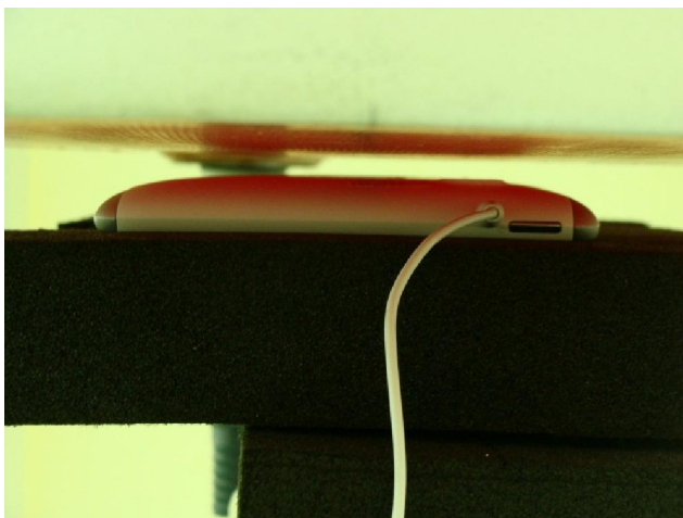
Rear Face of the DUT with Phantom 0.5 cm Gap
