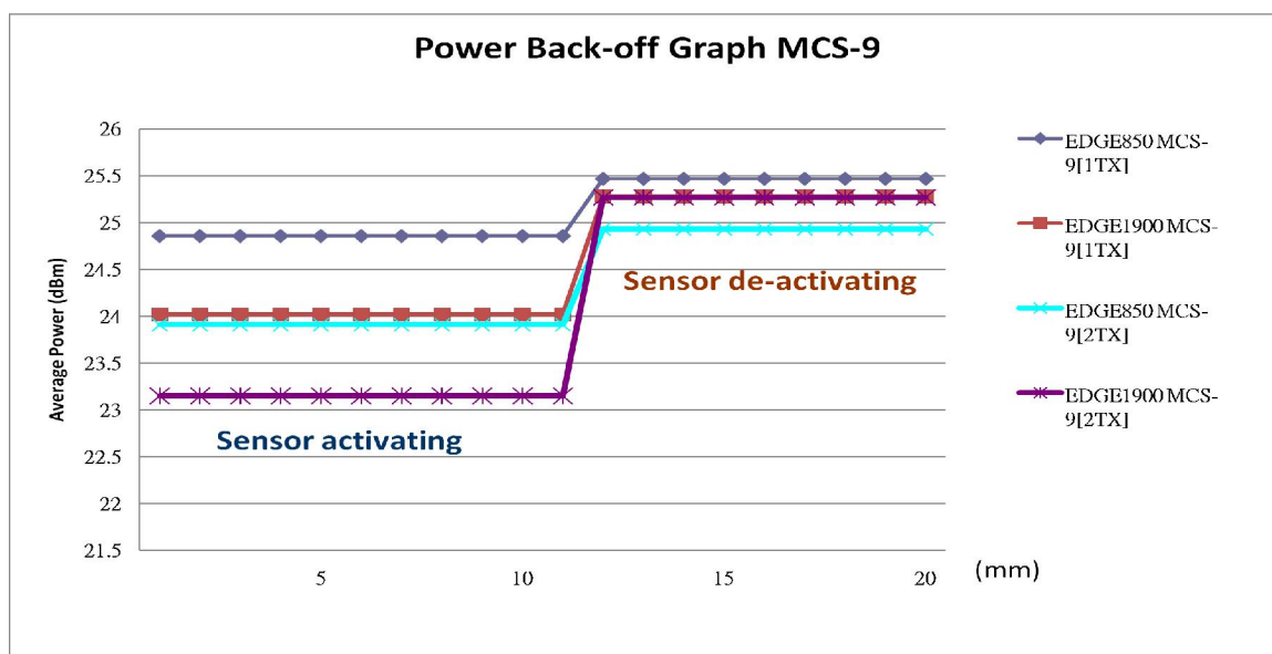
Power back- off Chart for E-GPRS 850/1900 (MCS-9)
