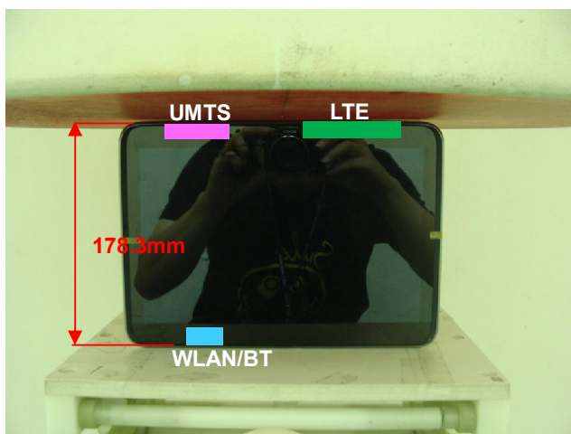
Secondary Landscape with Phantom 0 cm Gap for LTE and 2G/3G
