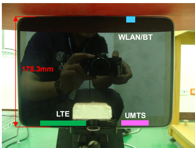
Primary Landscape with Phantom 0 cm Gap
