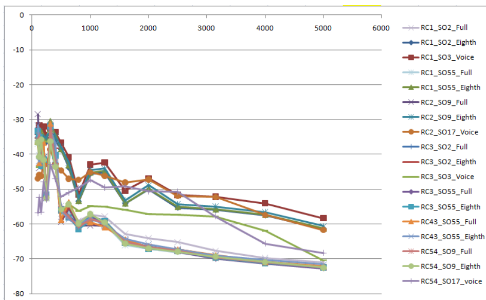
Fig. 5.10 Vocoder Analysis for ABM Noise
