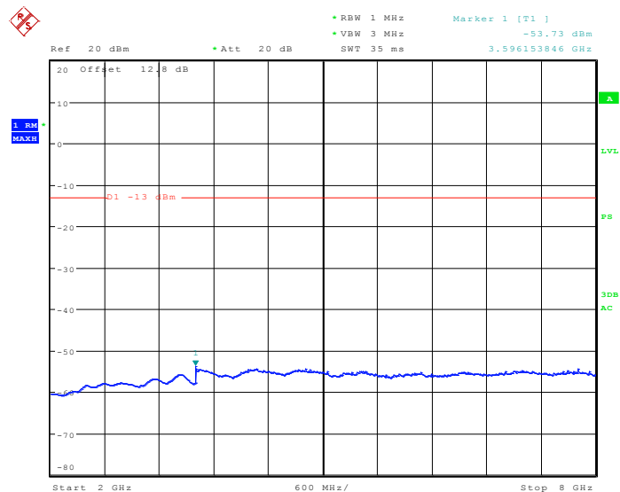
Conducted Emission Plot (2GHz ~ 8GHz) for QPSK (RB Size 1, RB Offset 49)
