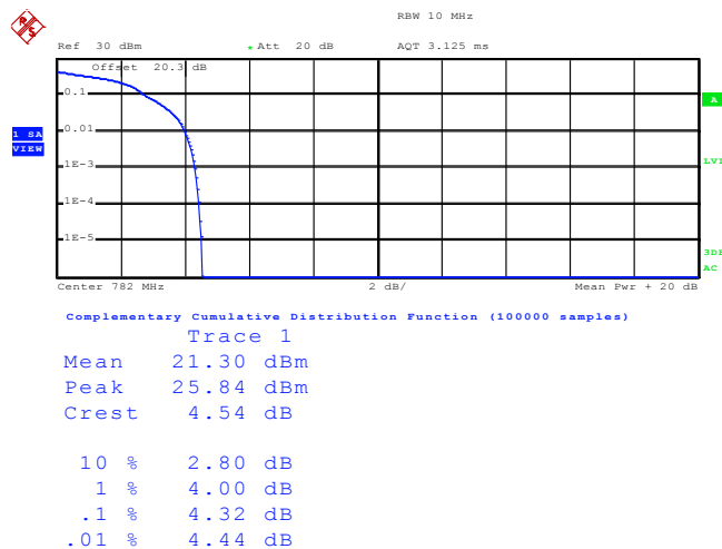
Peak-Average Ratio Plot for QPSK (RB Size 1, RB Offset 49)
