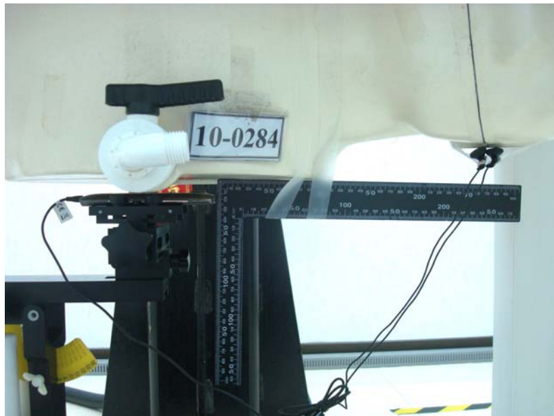
Body SAR Test Setup (Flat Section)
