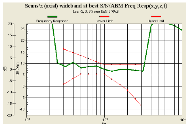
Fig. 9.5 GSM850 Ch128_Slide Off_Battery 1 (Phone 1)
