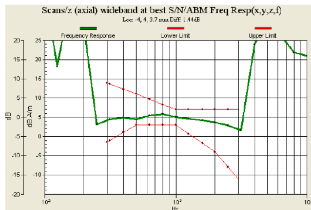
Fig. 9.3 GSM850 Ch128_Slide Off_Battery 2 (Phone 1)
