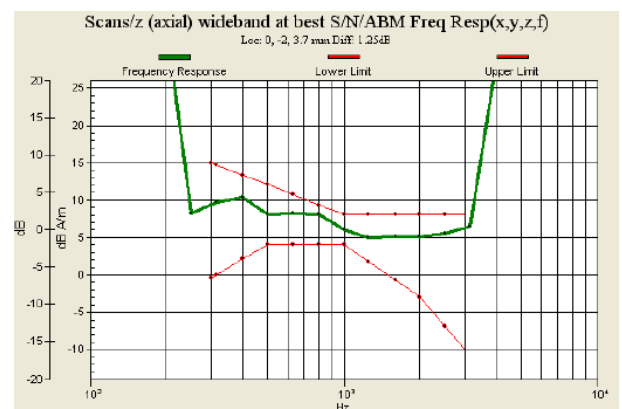
Fig. 9.24 WCDMA Band II Ch9400_Slide Left_Battery 1 (Phone 2)
