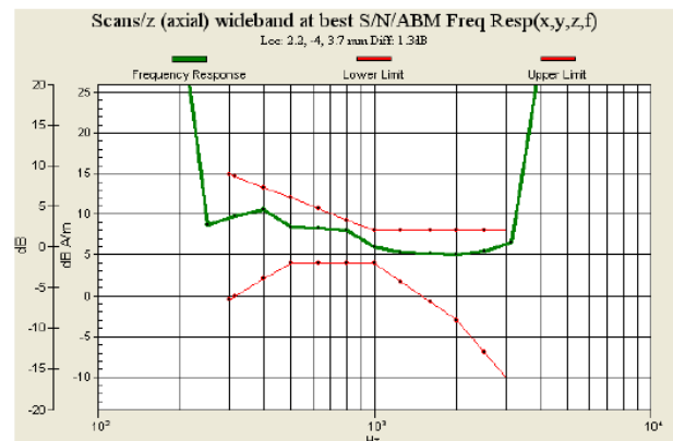
Fig. 9.18 WCDMA Band V Ch4233_Slide Left_Battery 1 (Phone 2)
