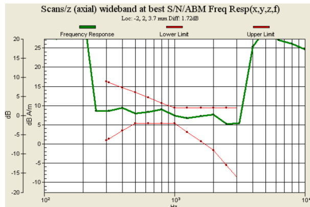
Fig. 9.1 GSM850 Ch189_Slide Off_Battery 2 (Phone 1)
