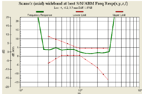
Fig. 9.13 WCDMA Band V Ch4182_Slide Off_Battery 2 (Phone 1)
