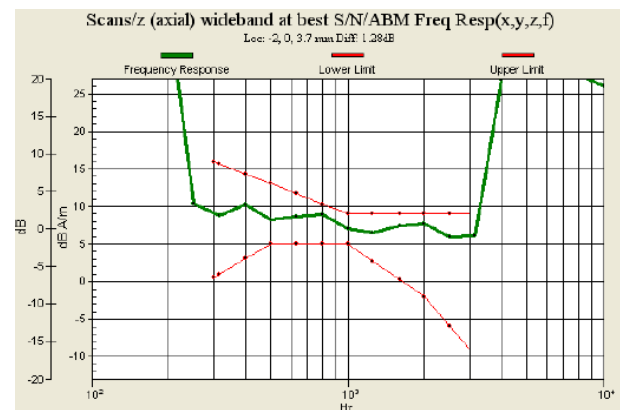
Fig. 9.4 GSM850 Ch251_Slide Off_Battery 2 (Phone 1)
