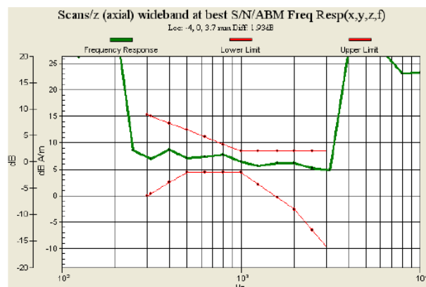
Fig. 9.11 GSM1900 Ch661_Slide Off_Battery 1 (Phone 1)
