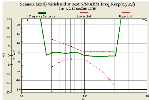
Fig. 9.15 WCDMA Band V Ch4132_Slide Left_Battery 2 (Phone 1)
