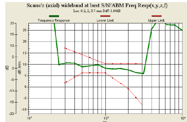
Fig. 9.6 GSM850 Ch128_Slide Off_Battery 2 (Phone 2)
