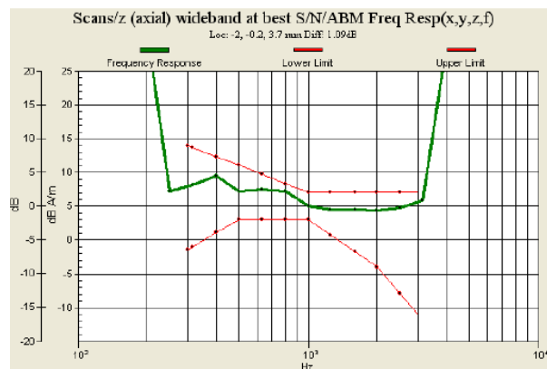
Fig. 9.21 WCDMA Band II Ch9262_Slide Left_Battery 2 (Phone 1)
