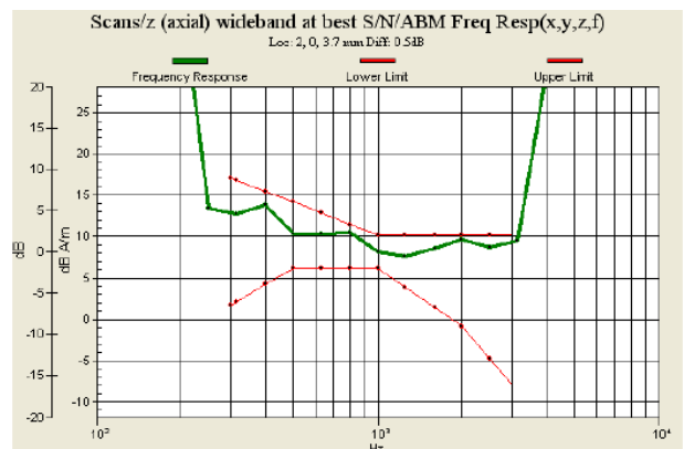
Fig. 9.12 GSM1900 Ch661_Slide Off_Battery 1 (Phone 2)
