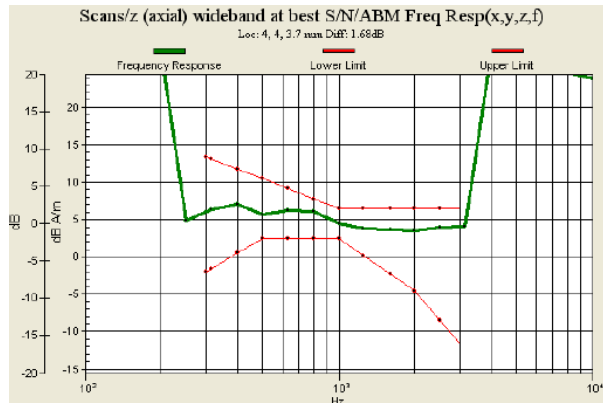
Fig. 9.19 WCDMA Band II Ch9400_Slide Off_Battery 2 (Phone 1)
