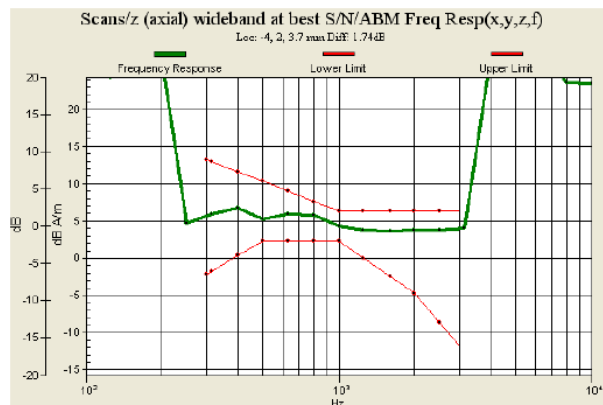
Fig. 9.17 WCDMA Band V Ch4233_Slide Left_Battery 1 (Phone 1)
