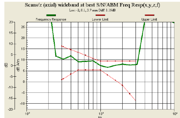
Fig. 9.2 GSM850 Ch189_Slide Left_Battery 2 (Phone 1)
