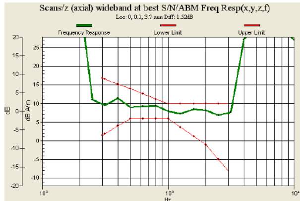
Fig. 9.7 GSM1900 Ch661_Slide Off_Battery 2 (Phone 1)
