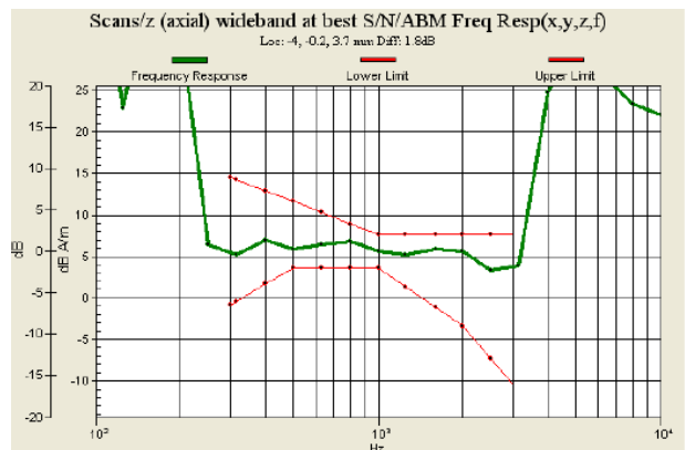
Fig. 9.10 GSM1900 Ch810_Slide Off_Battery 2 (Phone 1)
