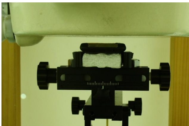
Face of the DUT with Phantom 1 cm Gap
