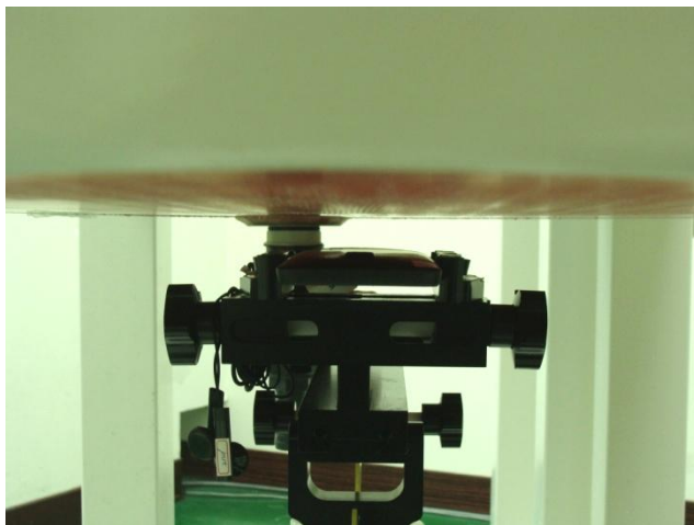
Bottom of the DUT with Phantom 1.5 cm Gap - Pocket PC Phone 2
