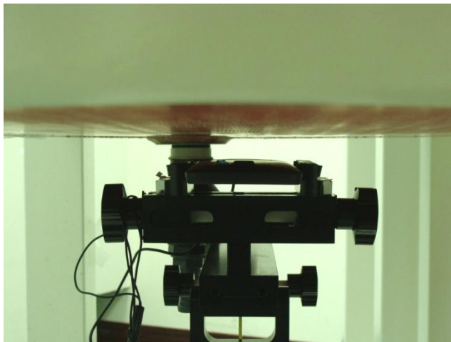
Bottom of the DUT with Phantom 1.5 cm Gap - Pocket PC Phone 1
