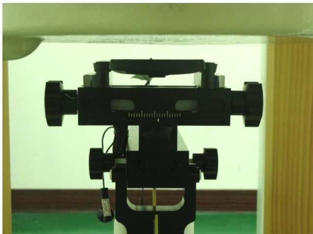
Face of the DUT with Phantom 1.5 cm Gap - Pocket PC Phone 2
