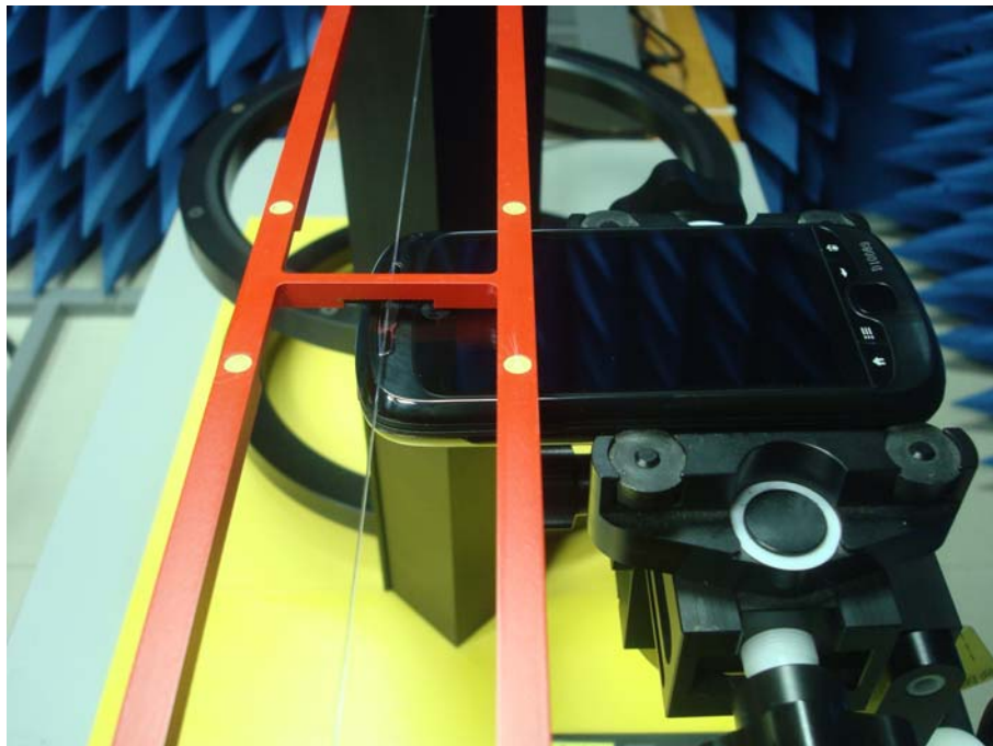
Figure 2. Setup Photo
