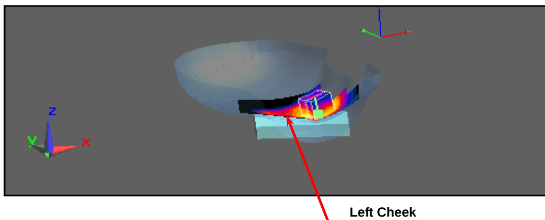
Figure 6. Left Head SAR Test Setup (Cheek)_Open
