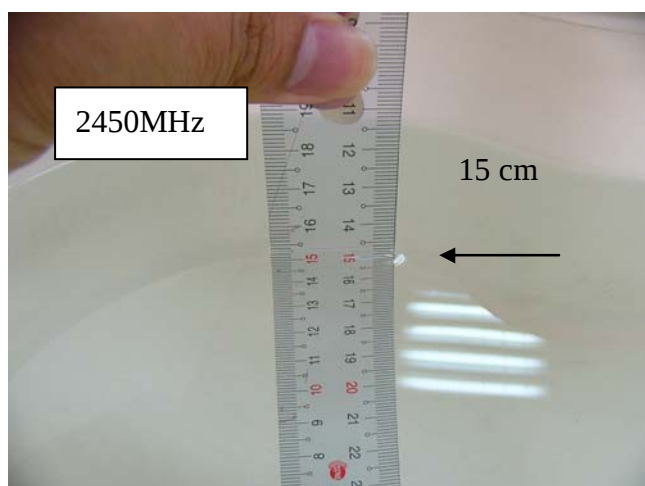
Fig.2.3 Photograph of the Tissue Simulant Fluid liquid depth 15cm for Right-head Side
