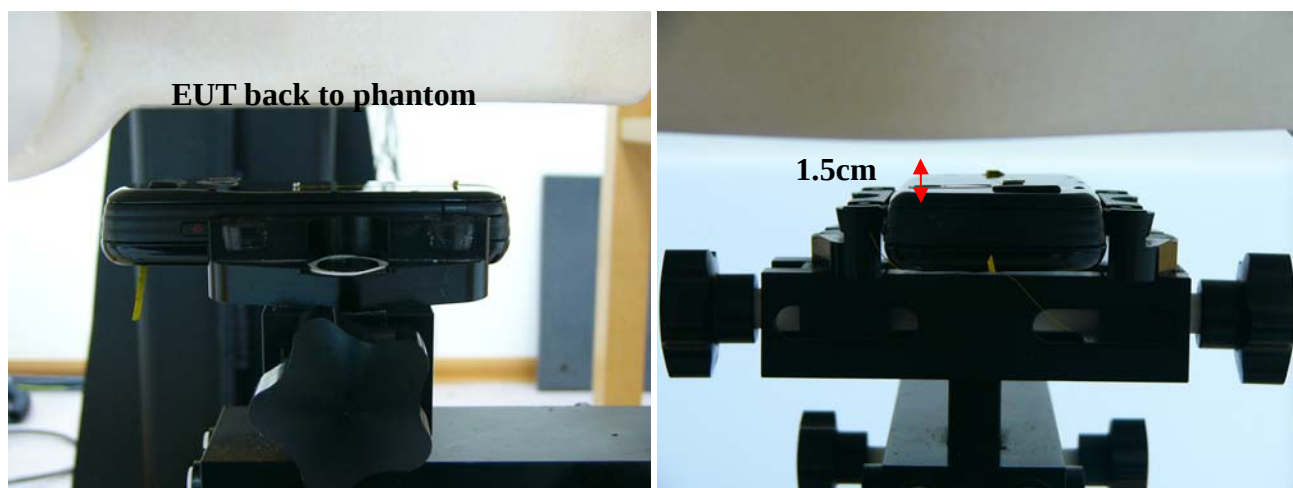
Fig.14 Body worn- EUT back to flat phantom and distance between flat phantom and mobile phone is 1.5 cm
