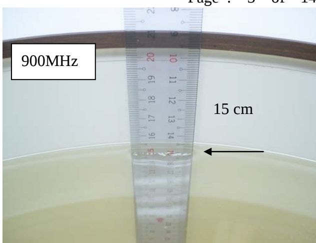
Fig.2.4 Photograph of the Tissue Simulant Fluid liquid depth 15cm for Flat (Body)
