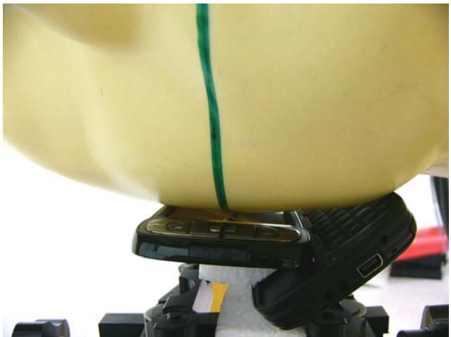
Fig.5 Right Head at Hold up Section / Cheek-Touch Position
