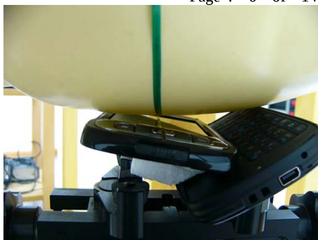
Fig.10 Left Head at Hold up Section / Cheek-Touch Position
