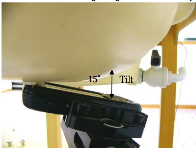
Fig.6 Right Head at Slider-off Section / Ear-Tilt Position( 15^{\circ} )
