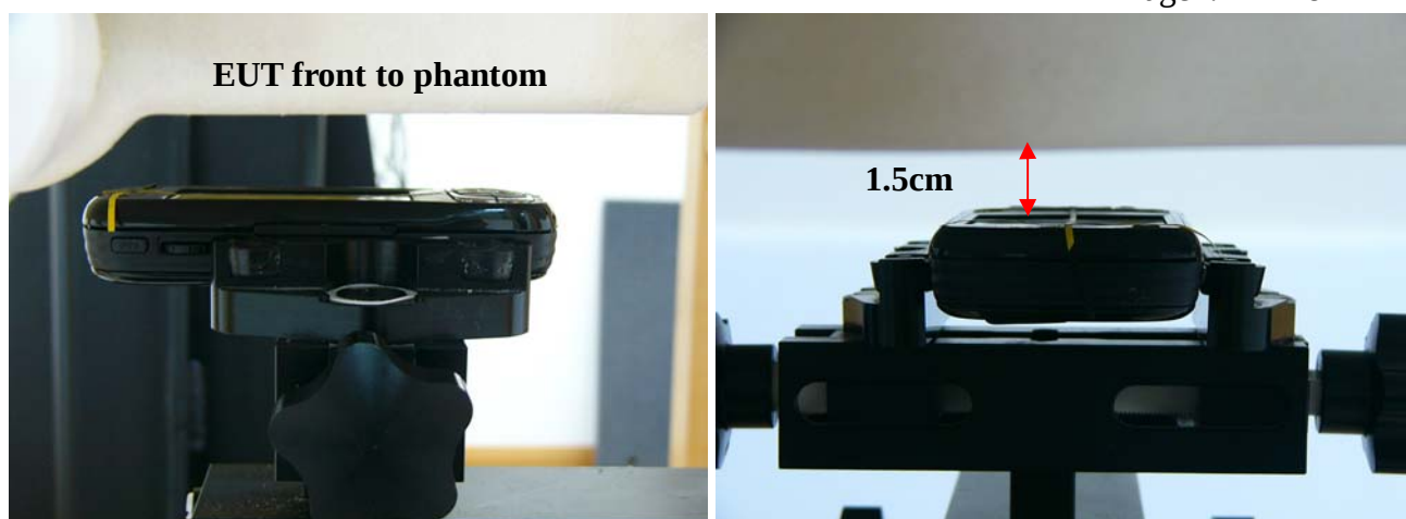
Fig.13 Body worn- EUT front to flat phantom and distance between flat phantom and mobile phone is 1.5 cm
