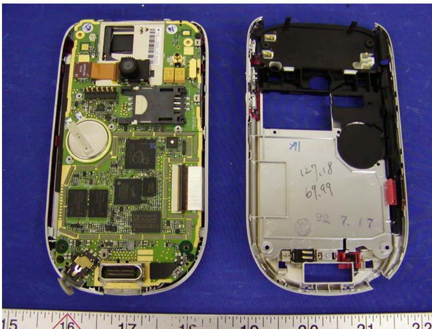
EUT – PH10A/PH10B Chassis Cover Off View
