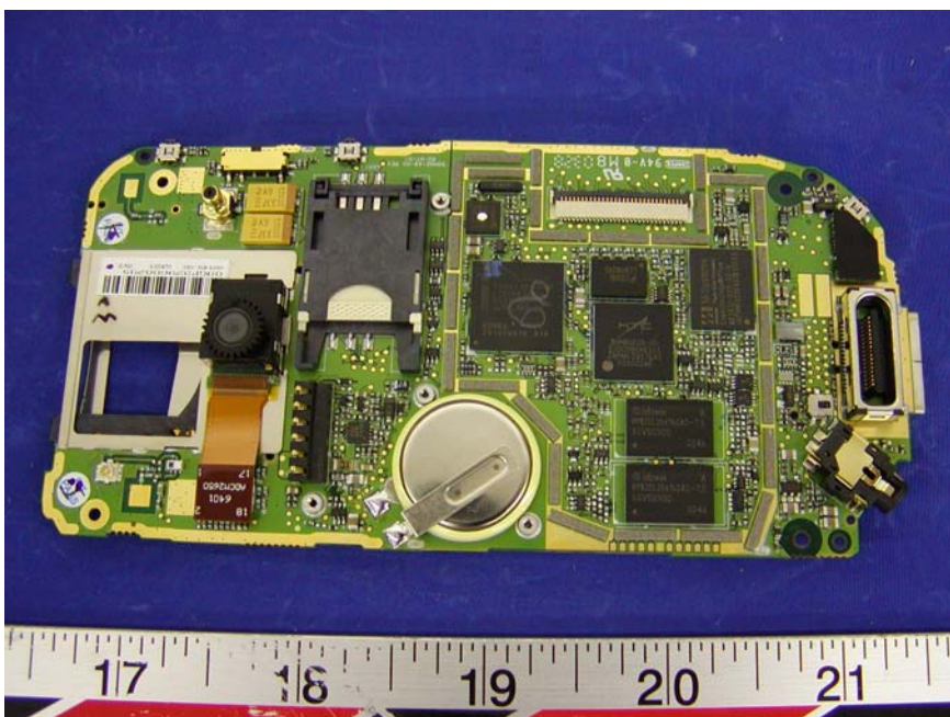
EUT – PH10A/PH10B Component View
