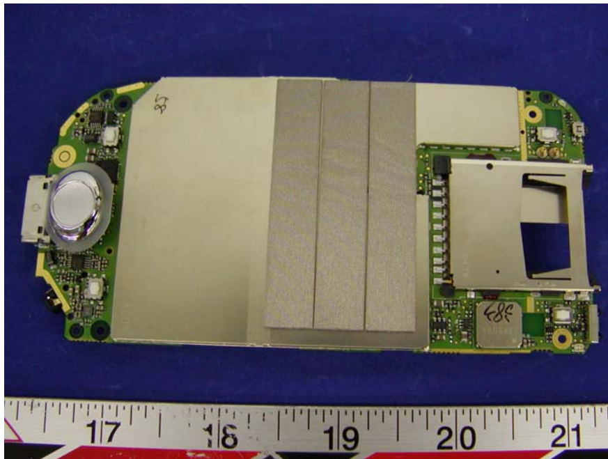
EUT – PH10A/PH10B Solder View with Shield
