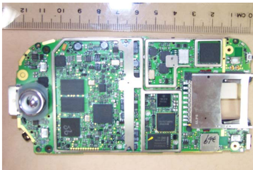
EUT – PH10A/PH10B Solder View without Shield
