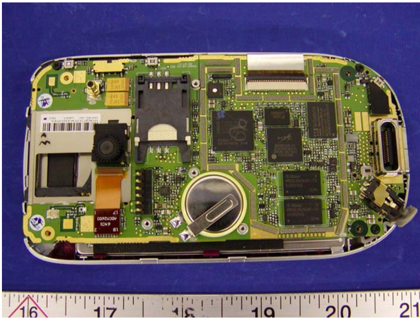
EUT – PH10A/PH10B Component View with Housing
