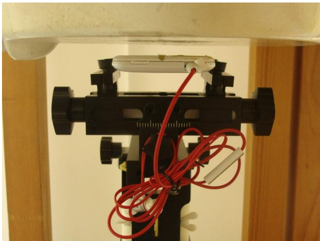
Front of the DUT with Phantom 1 cm Gap (DUT with Headset)
