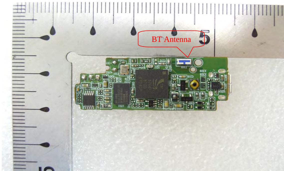
Antenna location
