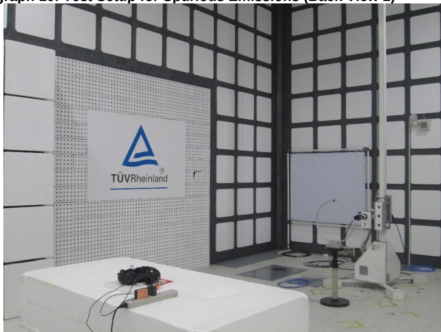
Photograph 10: Test Setup for Spurious Emissions (Back View 1)
