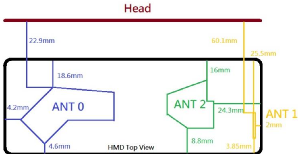
Photograph 7. Antenna position of EUT - End of Report -
