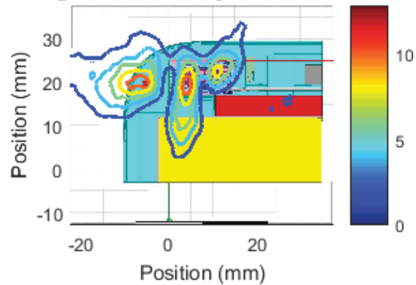
Right Module , Channel 2, front Cut Sector 22 Near Field Pattern Average Power Density: 4.85 W/m 2 over 4 cm 2
