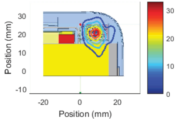
Left Module , Channel 1, front Cut Sector 2 Near Field Pattern Average Power Density: 8.79 W/m 2 over 4 cm 2
