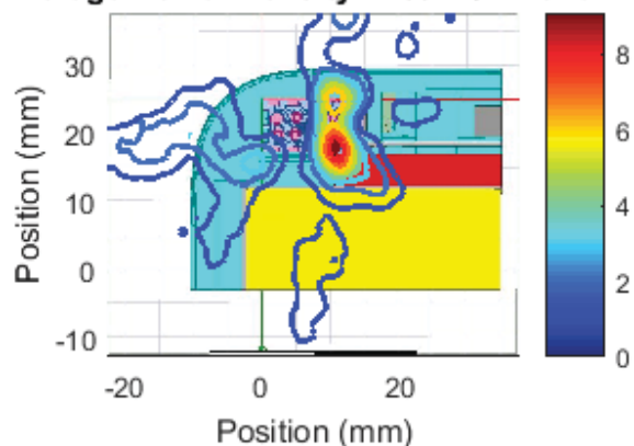
Right Module , Channel 2, front Cut Sector 15 Near Field Pattern Average Power Density: 2.09 W/m 2 over 4 cm 2
