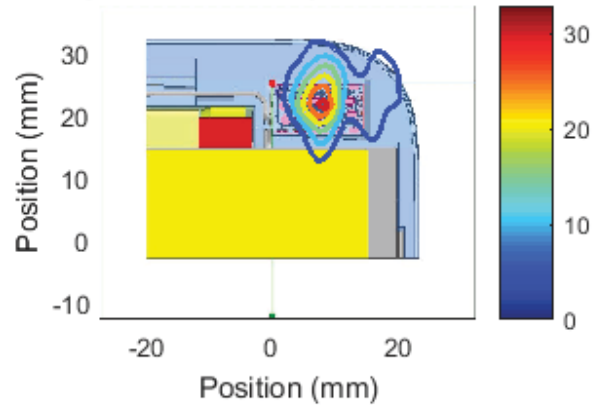
Left Module , Channel 2, front Cut Sector 3 Near Field Pattern Average Power Density: 7.37 W/m 2 over 4 cm 2
