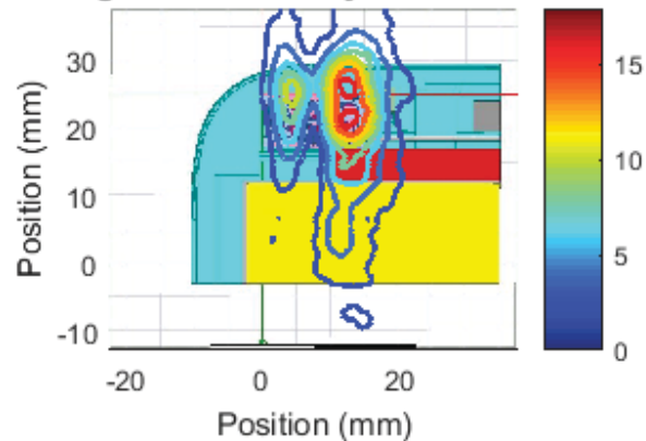
Right Module , Channel 3, front Cut Sector 15 Near Field Pattern Average Power Density: 6.5 W/m 2 over 4 cm 2
