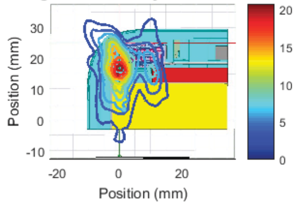
Right Module , Channel 2, front Cut Sector 13 Near Field Pattern Average Power Density: 2.36 W/m 2 over 4 cm 2
