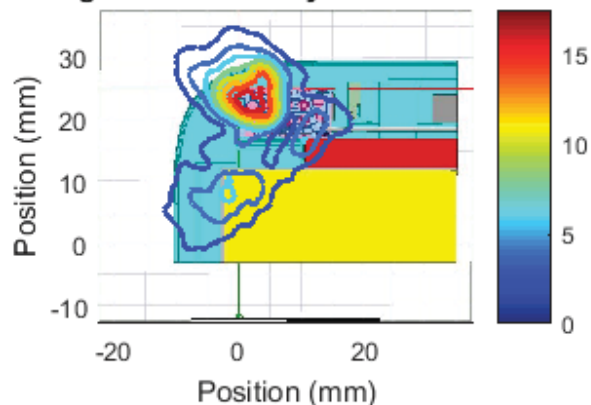
Right Module , Channel 3, front Cut Sector 7 Near Field Pattern Average Power Density: 5.35 W/m 2 over 4 cm 2
