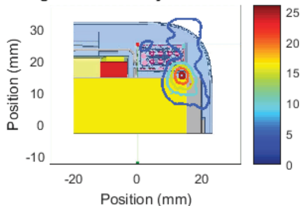
Left Module , Channel 3, front Cut Sector 19 Near Field Pattern Average Power Density: 6.64 W/m 2 over 4 cm 2
