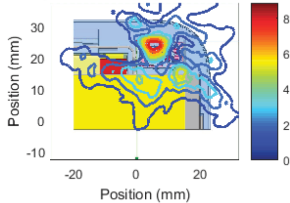
Left Module , Channel 4, front Cut Sector 21 Near Field Pattern Average Power Density: 7.91 W/m 2 over 4 cm 2
