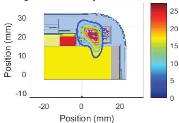
Left Module , Channel 2, front Cut Sector 8 Near Field Pattern Average Power Density: 7.53 W/m 2 over 4 cm 2
