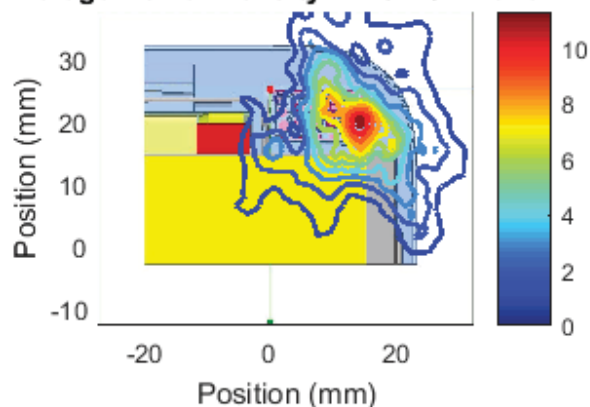
Left Module , Channel 3, front Cut Sector 22 Near Field Pattern Average Power Density: 4.43 W/m 2 over 4 cm 2
