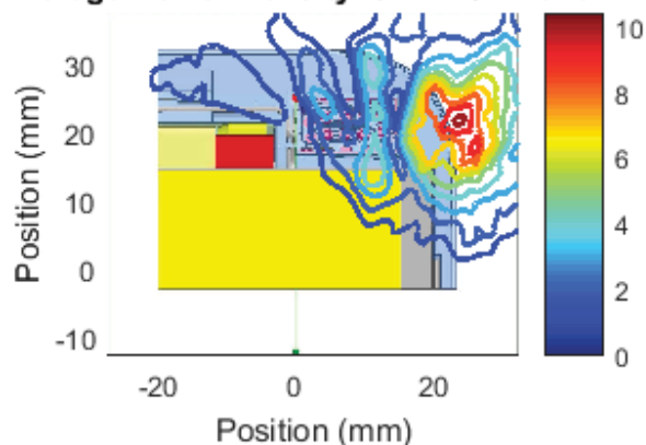
Left Module , Channel 2, front Cut Sector 0 Near Field Pattern Average Power Density: 5.12 W/m 2 over 4 cm 2
