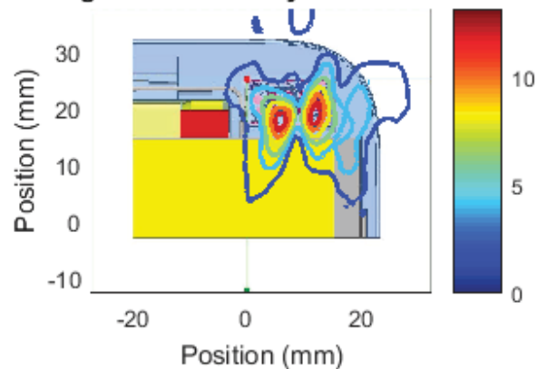
Left Module , Channel 4, front Cut Sector 1 Near Field Pattern Average Power Density: 4.6 W/m 2 over 4 cm 2
