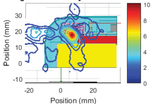
Right Module , Channel 1, front Cut Sector 26 Near Field Pattern Average Power Density: 2.22 W/m 2 over 4 cm 2
