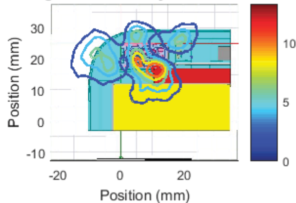
Right Module , Channel 4, front Cut Sector 4 Near Field Pattern Average Power Density: 4.3 W/m 2 over 4 cm 2
