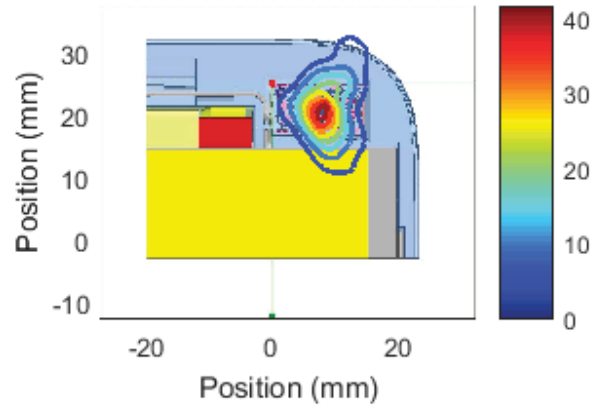
Left Module , Channel 4, front Cut Sector 8 Near Field Pattern Average Power Density: 8.16 W/m 2 over 4 cm 2
