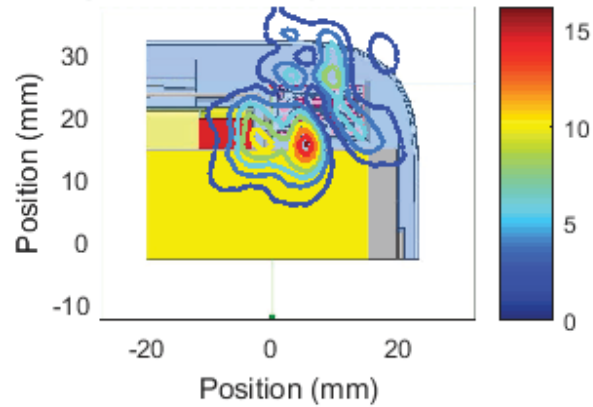
Left Module , Channel 4, front Cut Sector 13 Near Field Pattern Average Power Density: 2.63 W/m 2 over 4 cm 2
