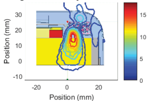
Left Module , Channel 2, front Cut Sector 5 Near Field Pattern Average Power Density: 5.96 W/m 2 over 4 cm 2
