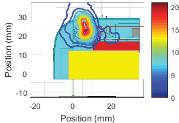
Right Module , Channel 3, front Cut Sector 3 Near Field Pattern Average Power Density: 6.49 W/m 2 over 4 cm 2
