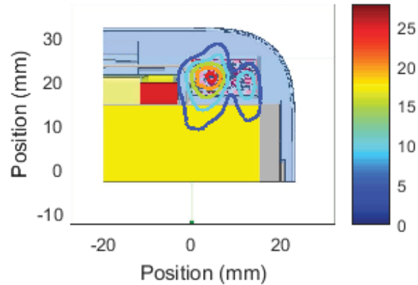
Left Module , Channel 3, front Cut Sector 31 Near Field Pattern Average Power Density: 7.68 W/m 2 over 4 cm 2
