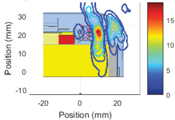
Left Module , Channel 2, front Cut Sector 21 Near Field Pattern Average Power Density: 4.96 W/m 2 over 4 cm 2
