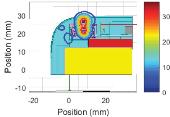
Right Module , Channel 4, front Cut Sector 17 Near Field Pattern Average Power Density: 7.84 W/m 2 over 4 cm 2
