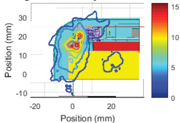
Right Module , Channel 4, front Cut Sector 31 Near Field Pattern Average Power Density: 5.61 W/m 2 over 4 cm 2
