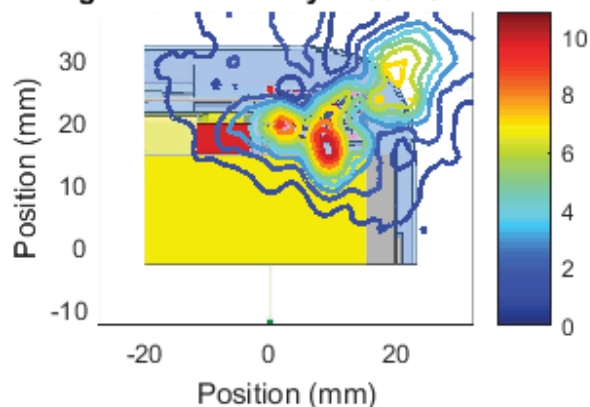
Left Module , Channel 2, front Cut Sector 24 Near Field Pattern Average Power Density: 4.33 W/m 2 over 4 cm 2
