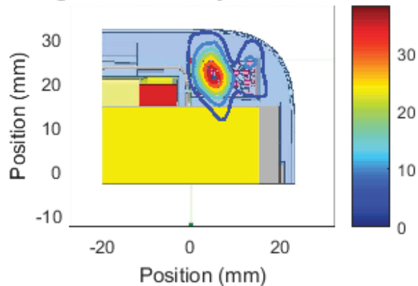
Left Module , Channel 4, front Cut Sector 4 Near Field Pattern Average Power Density: 8.33 W/m 2 over 4 cm 2
