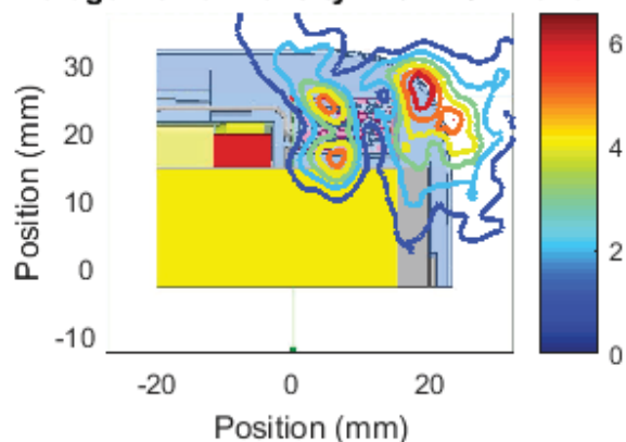
Left Module , Channel 3, front Cut Sector 1 Near Field Pattern Average Power Density: 2.91 W/m 2 over 4 cm 2
