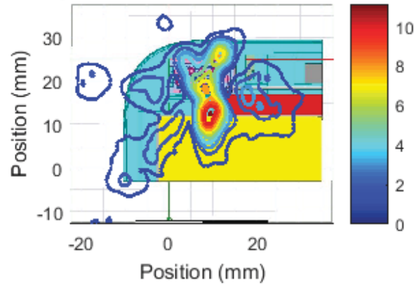
Right Module , Channel 1, front Cut Sector 18 Near Field Pattern Average Power Density: 7.33 W/m 2 over 4 cm 2
