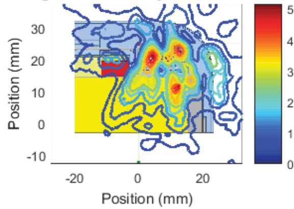
Left Module , Channel 2, front Cut Sector 31 Near Field Pattern Average Power Density: 5.17 W/m 2 over 4 cm 2
