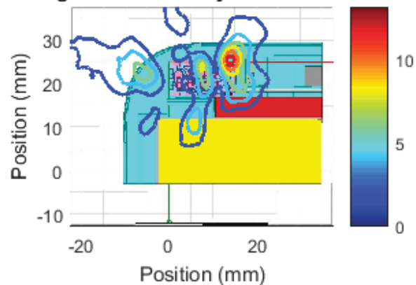
Right Module , Channel 2, front Cut Sector 14 Near Field Pattern Average Power Density: 3.31 W/m 2 over 4 cm 2
