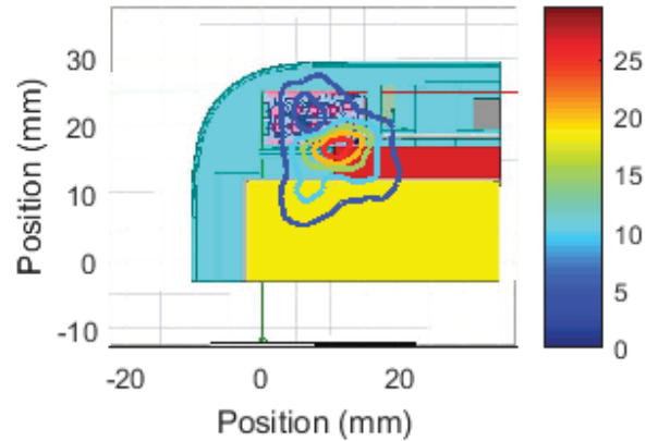
Right Module , Channel 3, front Cut Sector 13 Near Field Pattern Average Power Density: 7.77 W/m 2 over 4 cm 2
