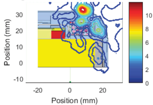
Left Module , Channel 3, front Cut Sector 25 Near Field Pattern Average Power Density: 3.31 W/m 2 over 4 cm 2
