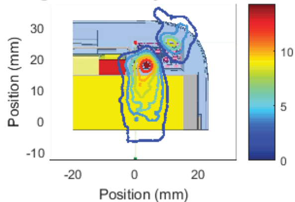
Left Module , Channel 4, front Cut Sector 10 Near Field Pattern Average Power Density: 4.62 W/m 2 over 4 cm 2
