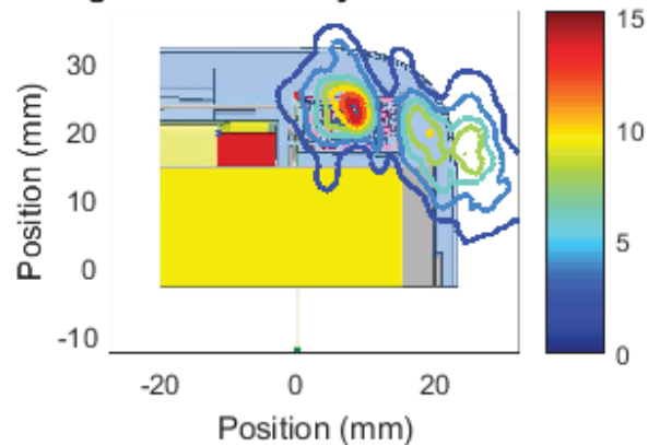
Left Module , Channel 3, front Cut Sector 27 Near Field Pattern Average Power Density: 4.66 W/m 2 over 4 cm 2
