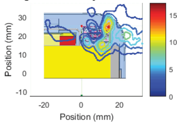
Left Module , Channel 3, front Cut Sector 0 Near Field Pattern Average Power Density: 5.49 W/m 2 over 4 cm 2
