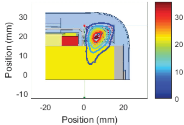
Left Module , Channel 3, front Cut Sector 28 Near Field Pattern Average Power Density: 8.42 W/m 2 over 4 cm 2
