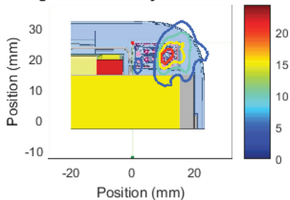
Left Module , Channel 3, front Cut Sector 4 Near Field Pattern Average Power Density: 7.53 W/m 2 over 4 cm 2
