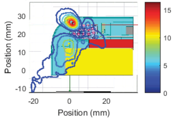
Right Module , Channel 1, front Cut Sector 4 Near Field Pattern Average Power Density: 2.88 W/m 2 over 4 cm 2
