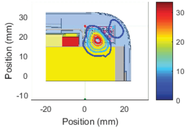
Left Module , Channel 1, front Cut Sector 8 Near Field Pattern Average Power Density: 7.78 W/m 2 over 4 cm 2
