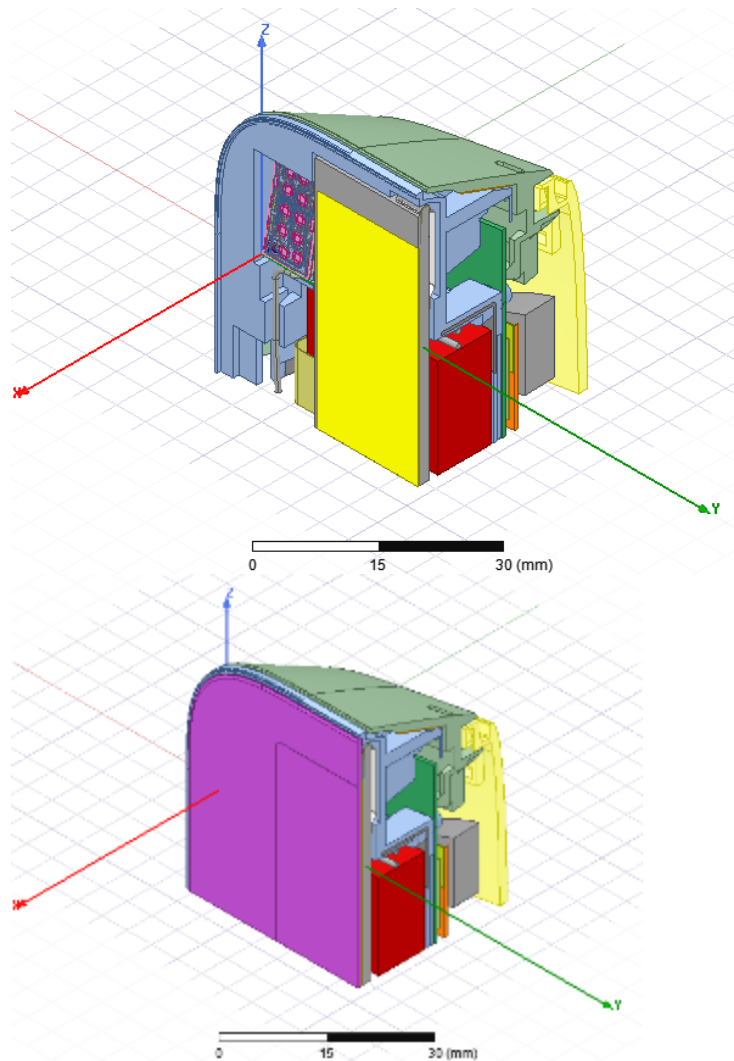
Figure C-4 Left module
