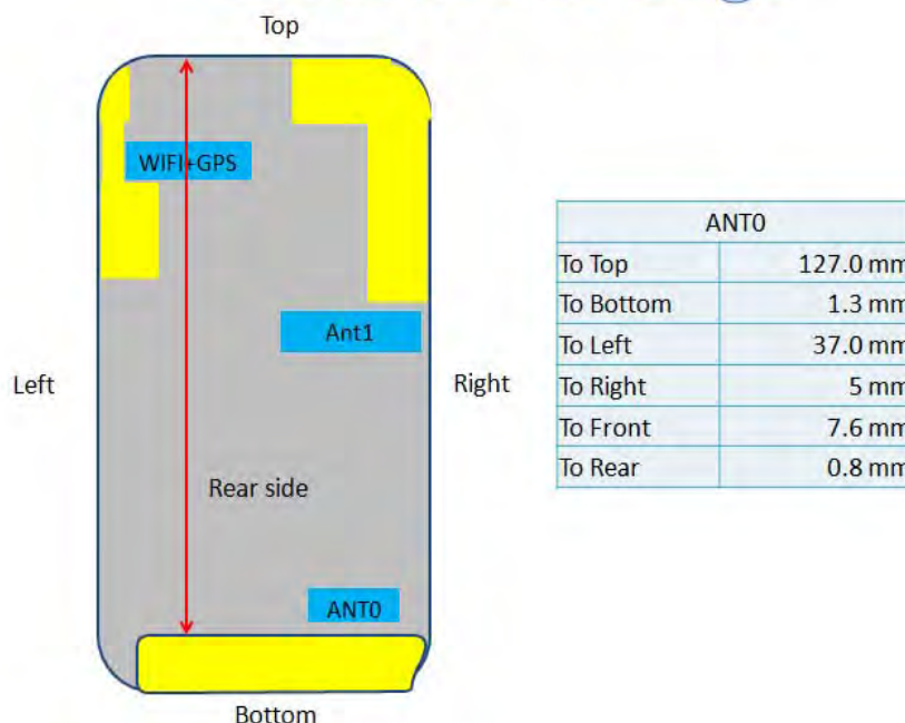
Fig.17 Antenna position of EUT
