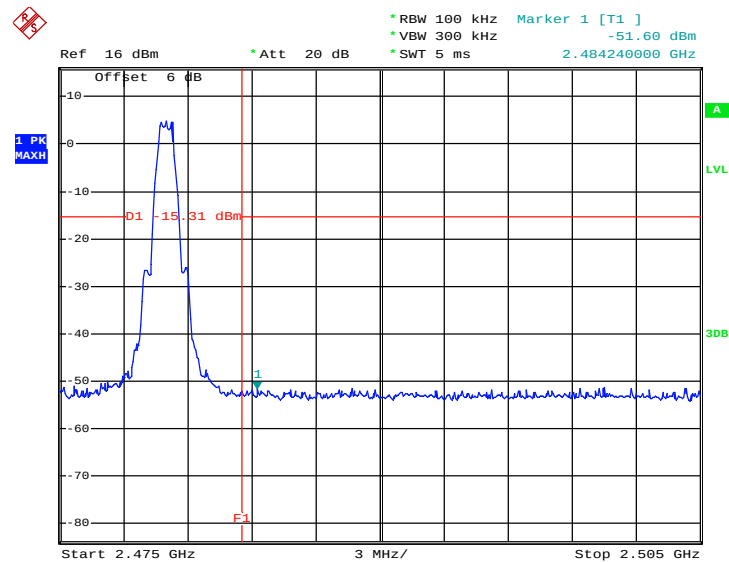
High Band Edge Plot on Channel 39
