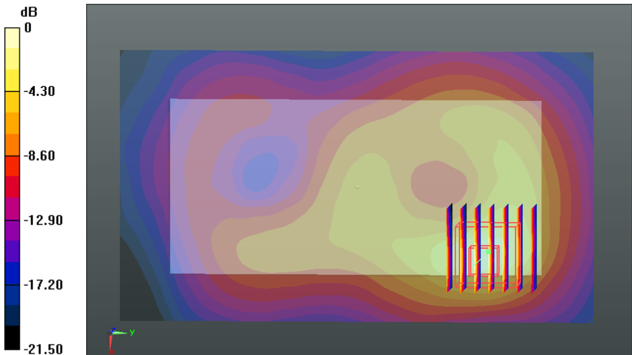
0 dB = 0.880mW/g
