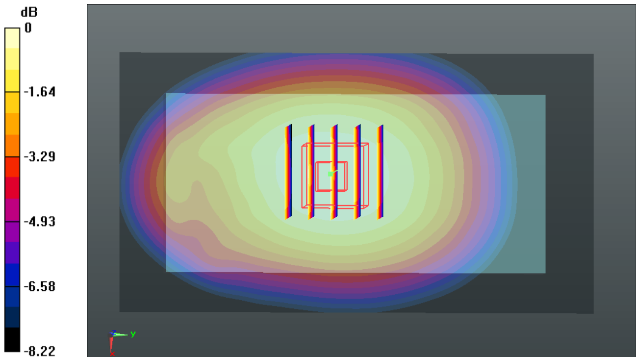
0 dB = 0.690\text{mW/g}
