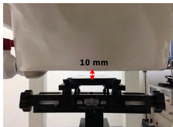
Fig.10 EUT front to flat phantom
