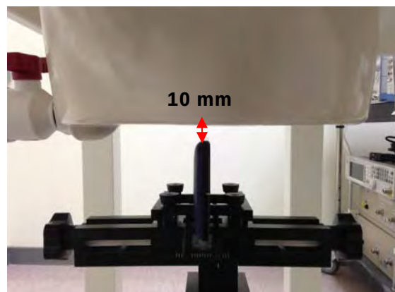
Fig.14 EUT left to flat phantom
