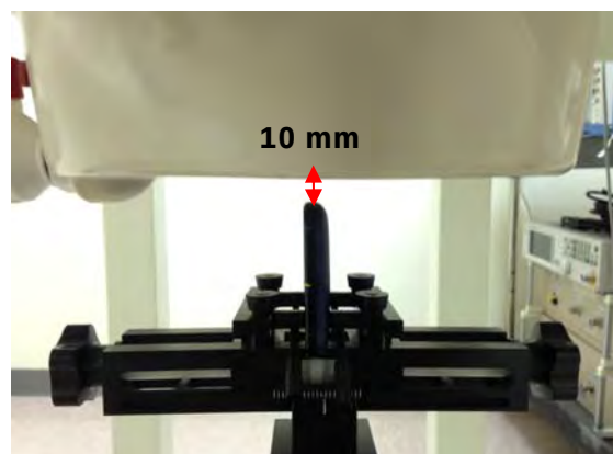
Fig.13 EUT right to flat phantom
