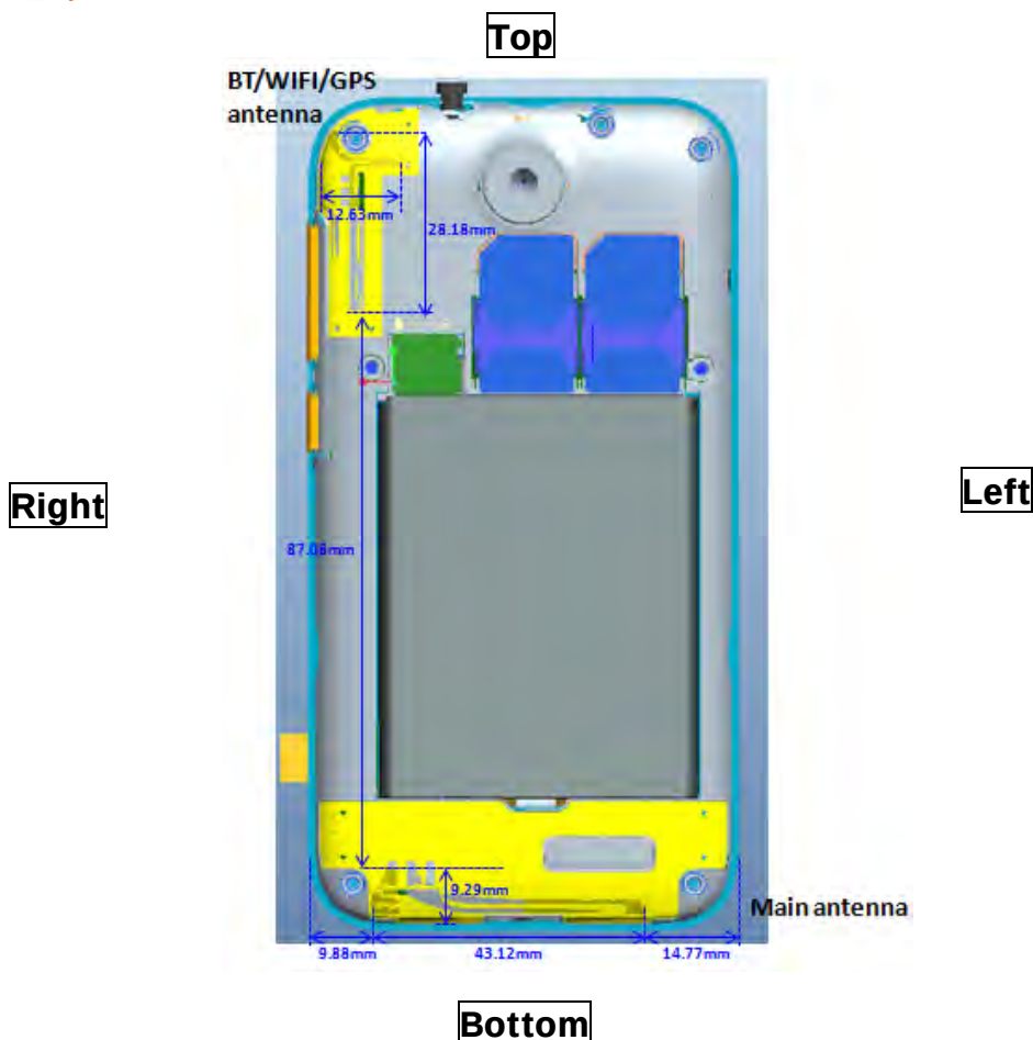
Fig.21 Antenna position of EUT (Back view)
