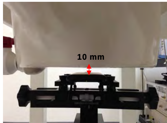
Fig.9 EUT back to flat phantom
