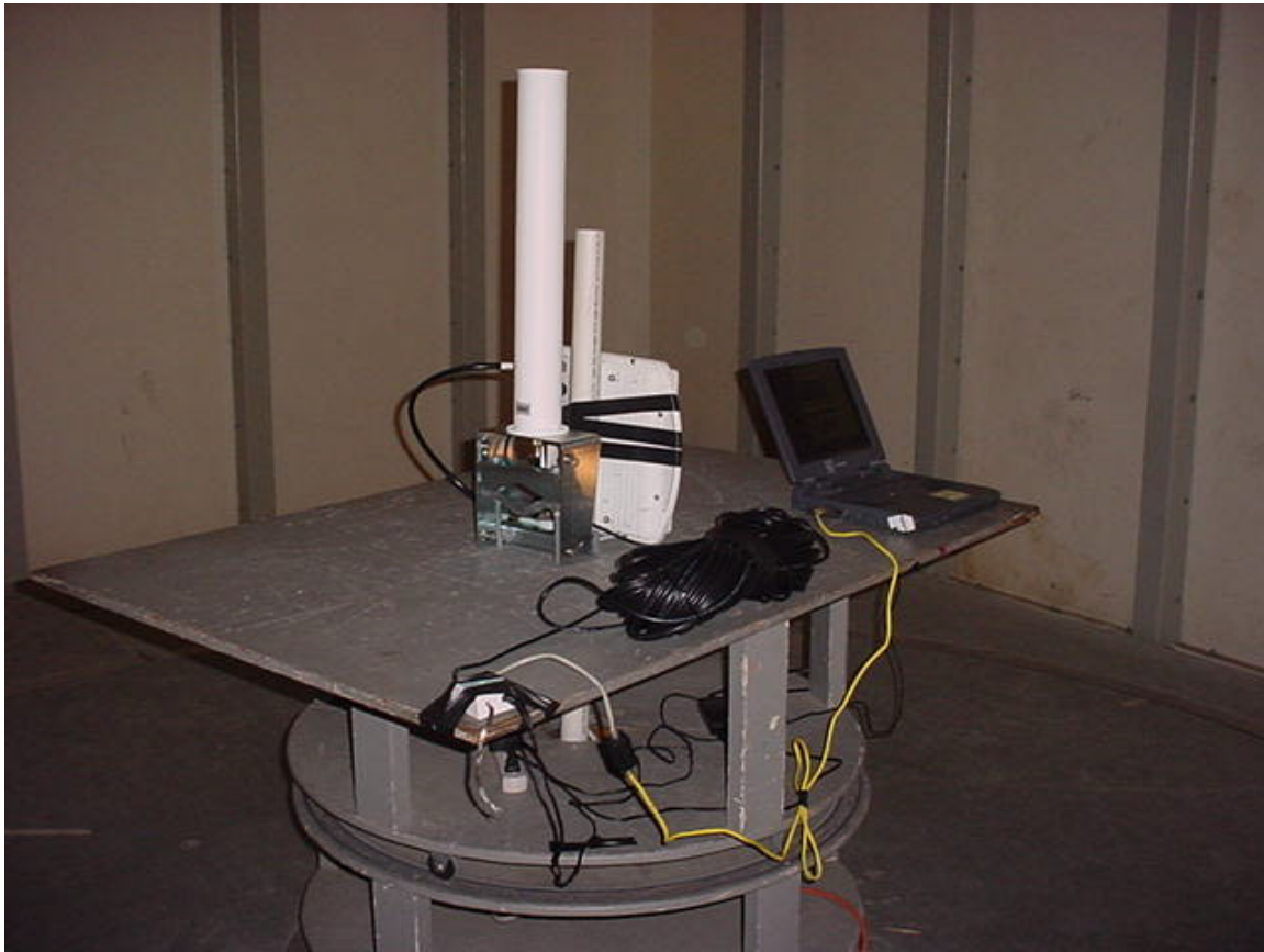
16dBi Sector Antenna Radiated Emissions
