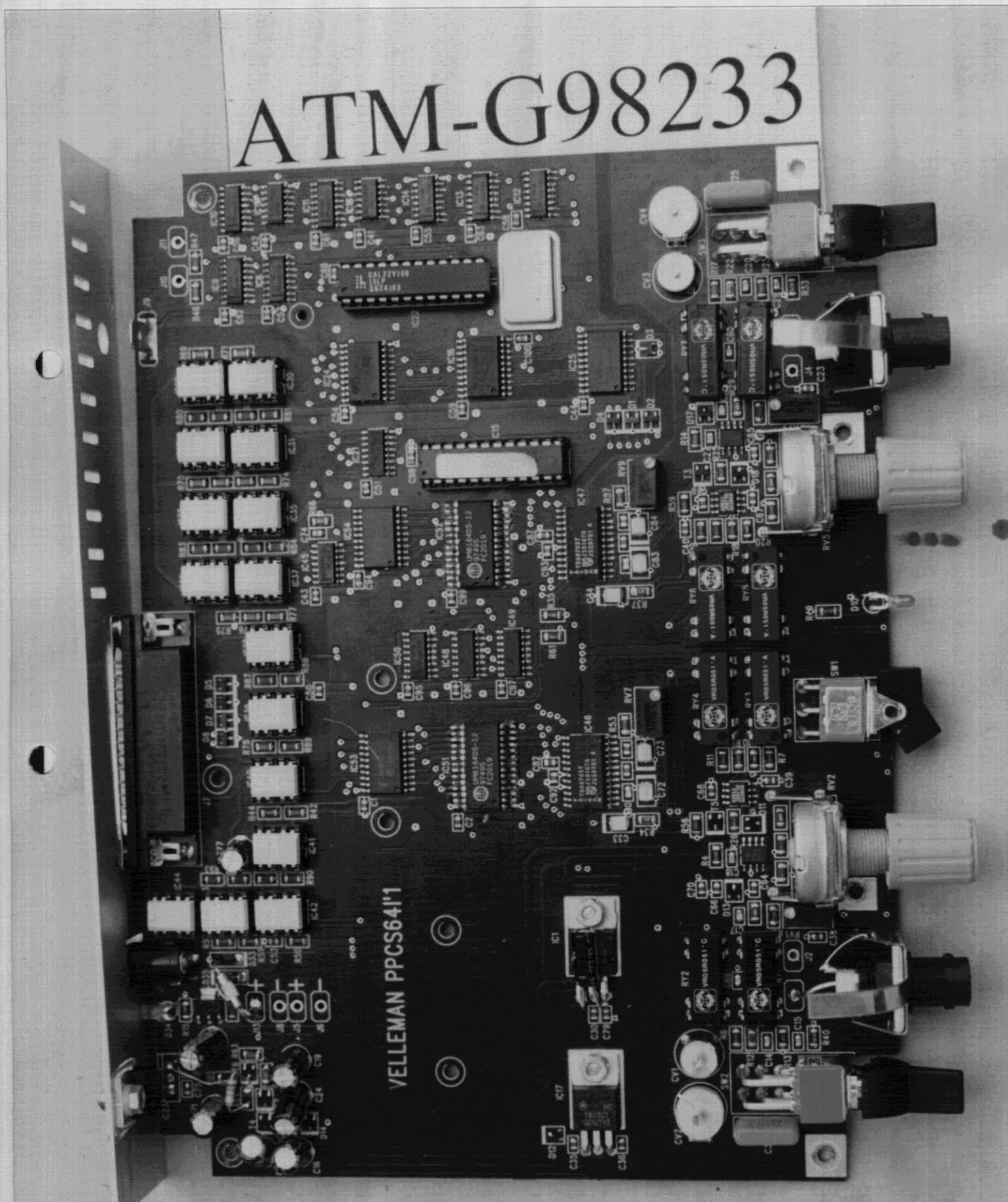
Figure 4 Main Board (Component Side)
