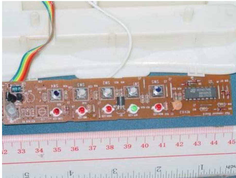
Control button PCB component side
