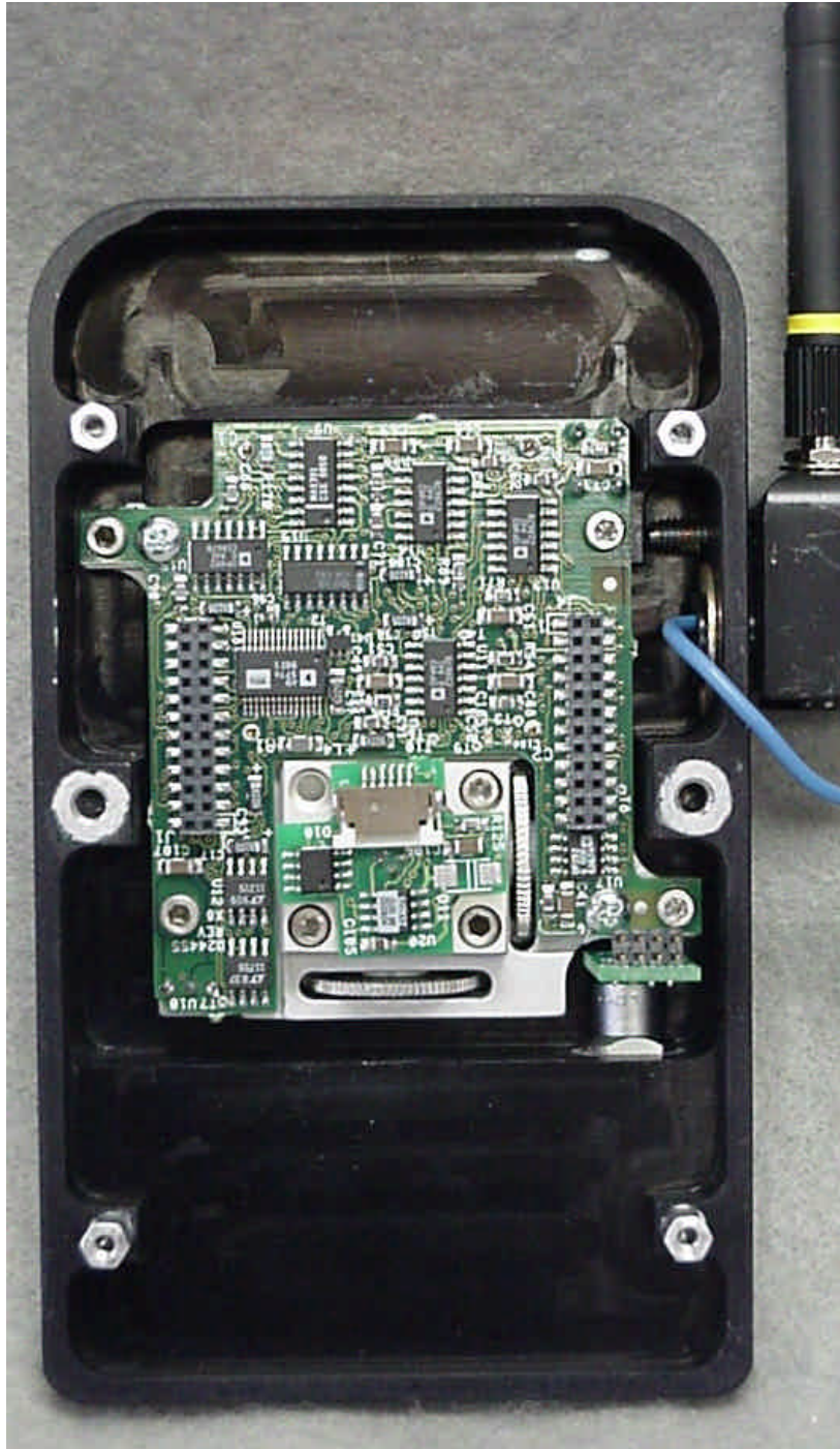
Photo 11. EUT, Laser Alignment Head CPU Board and TX Board Removed
