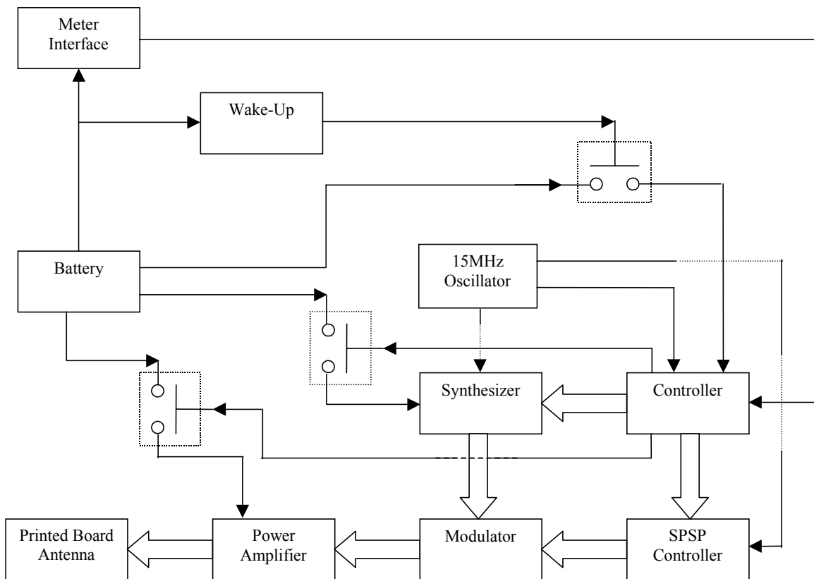
Figure 4. Block Diagram
