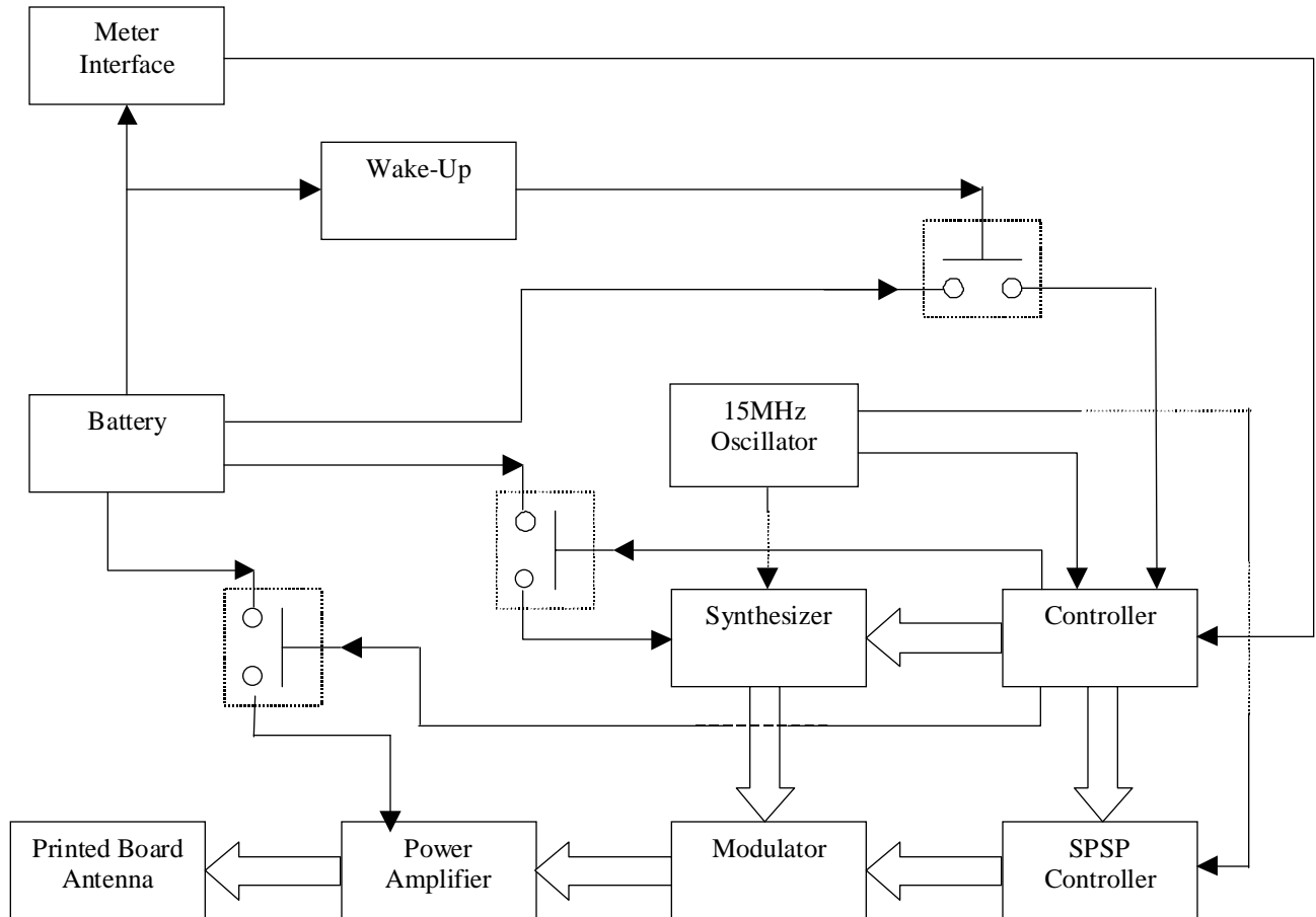
Figure 4. Block Diagram
