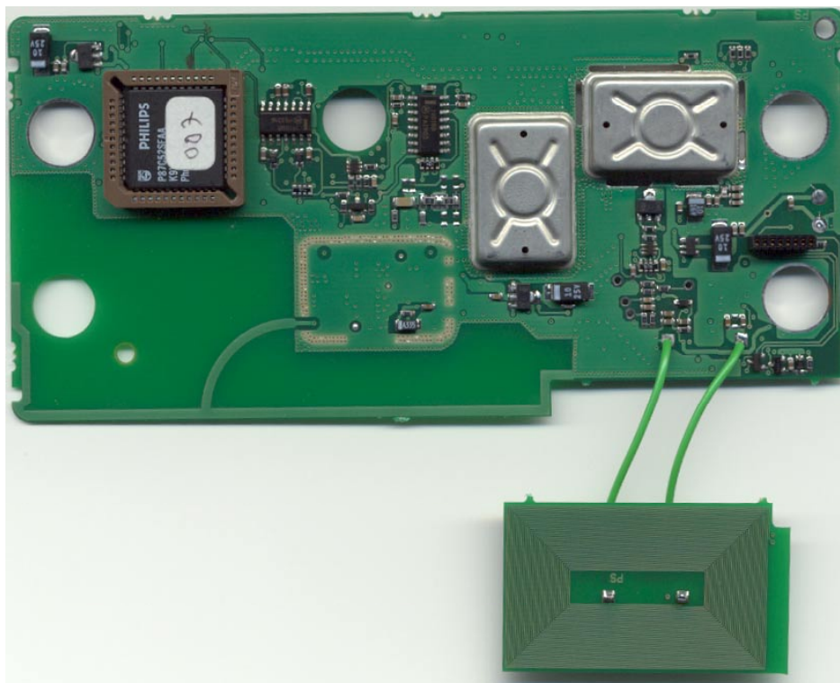
Figure 1 Printed Circuit Side 1
