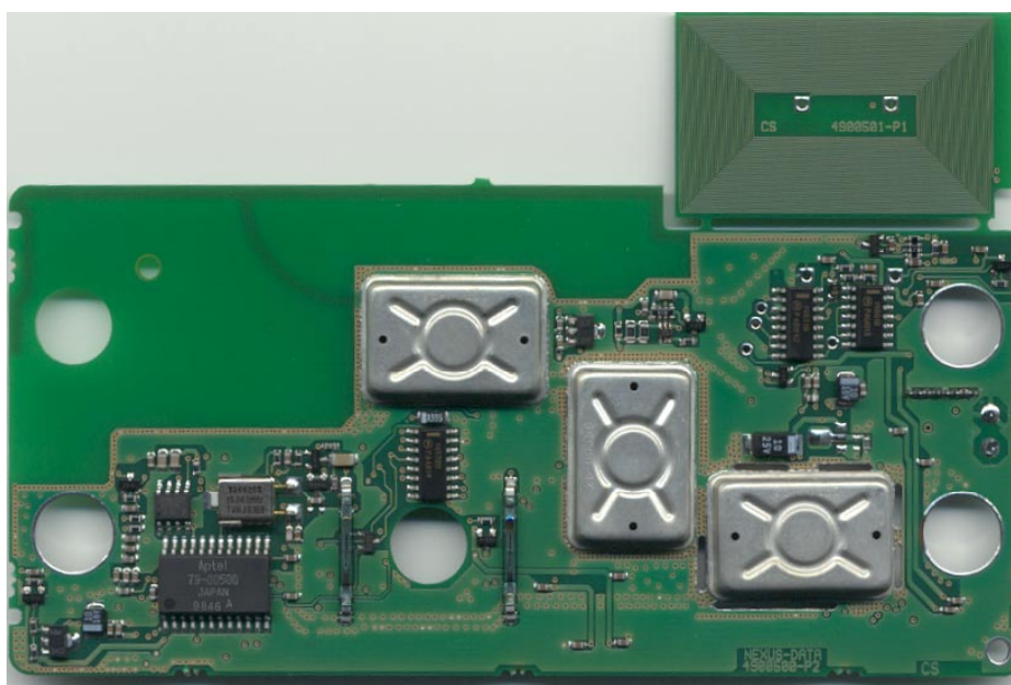
Figure 2 Printed Circuit Side 2
