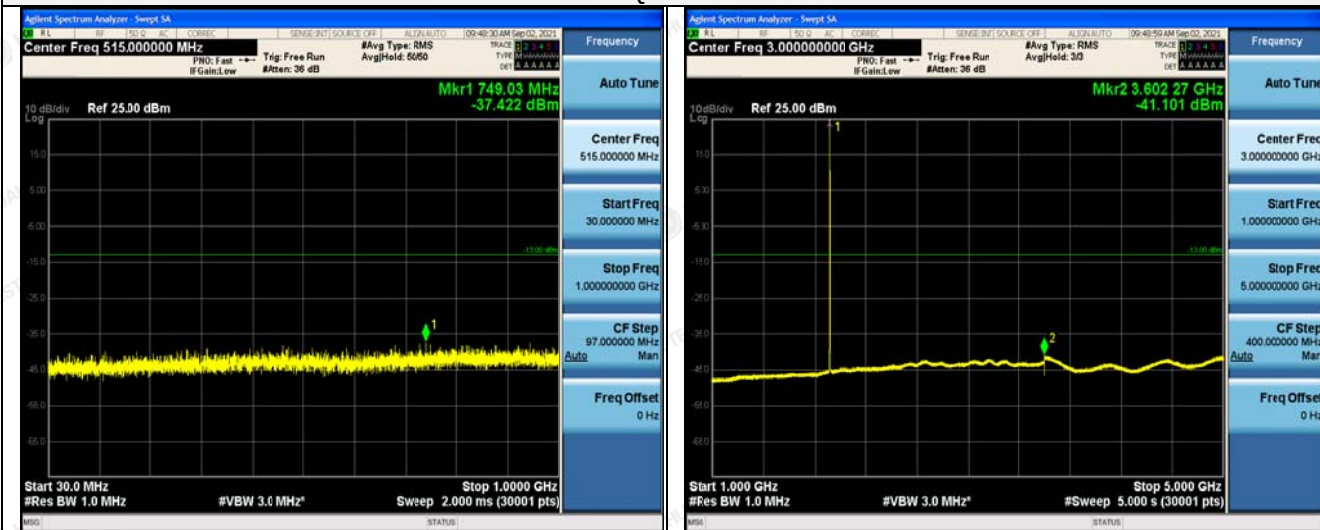
30MHz~1GHz
