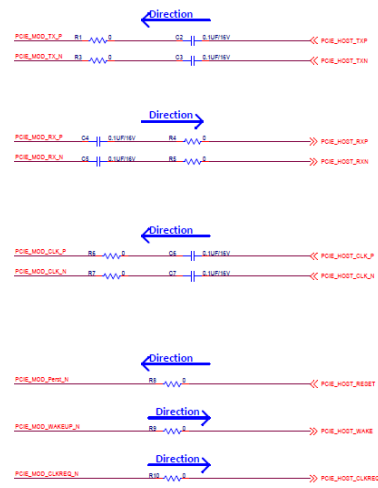
PCIe Interface
