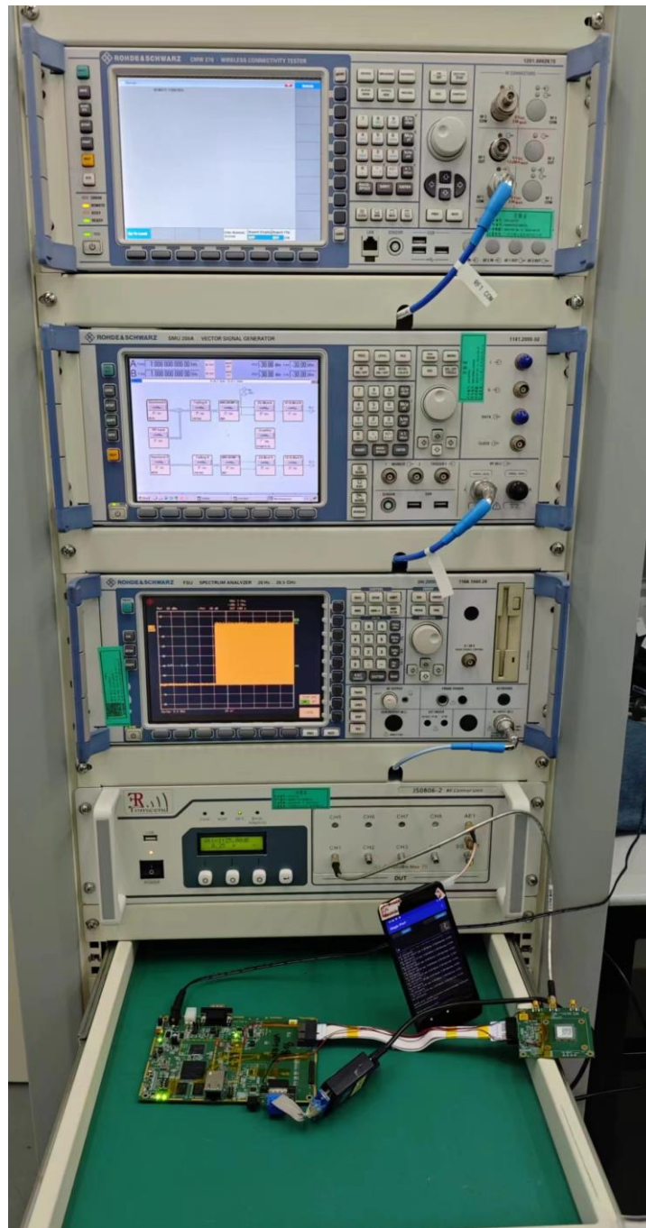
Figure: DFS Set-up Photo
