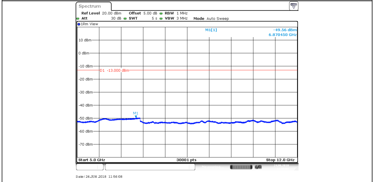
BAND 25_20MHz_16QAM_26590_1RB#0
