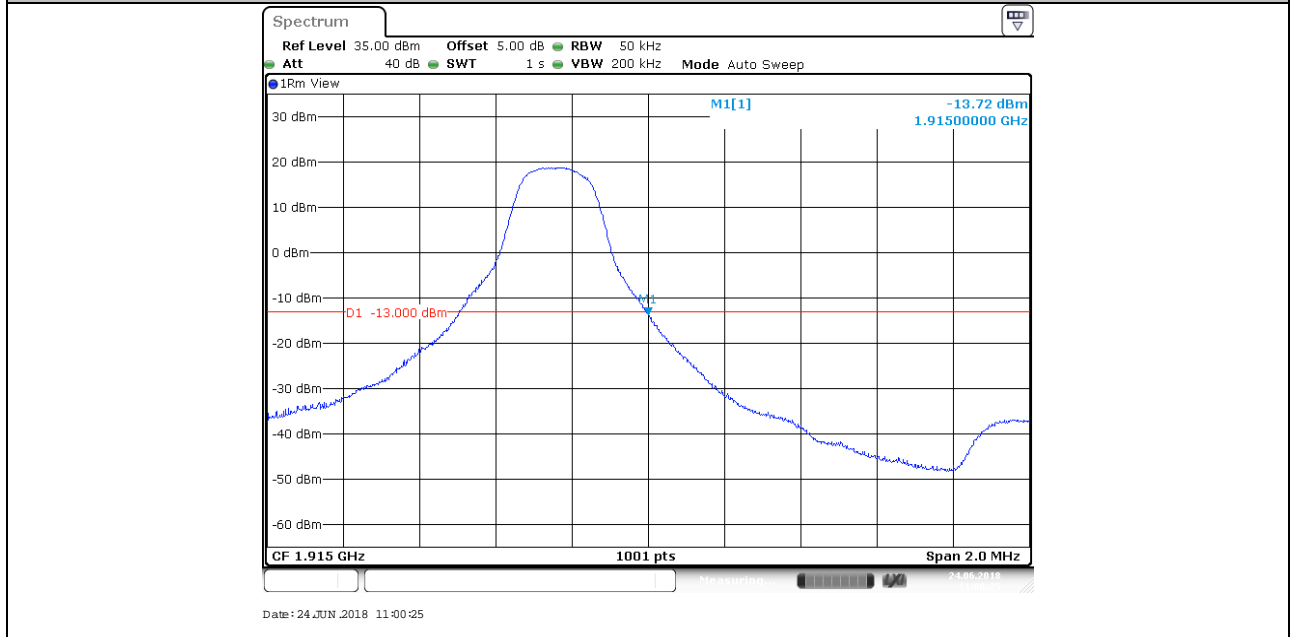
BAND 25_3MHz_QPSK_26675_15RB#0
