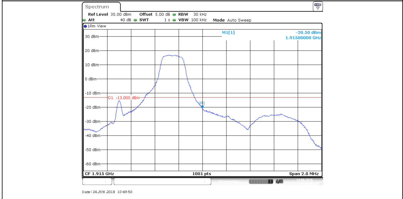
BAND 25_1.4MHz_QPSK_26683_6RB#0
