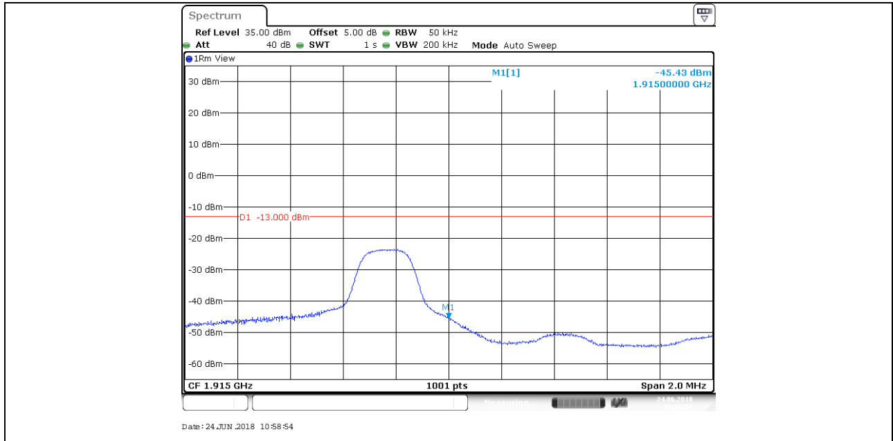
BAND 25_3MHz_QPSK_26675_1RB#14
