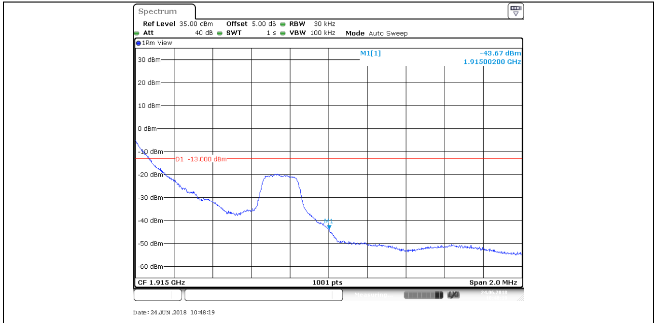
BAND 25_1.4MHz_QPSK_26683_1RB#5
