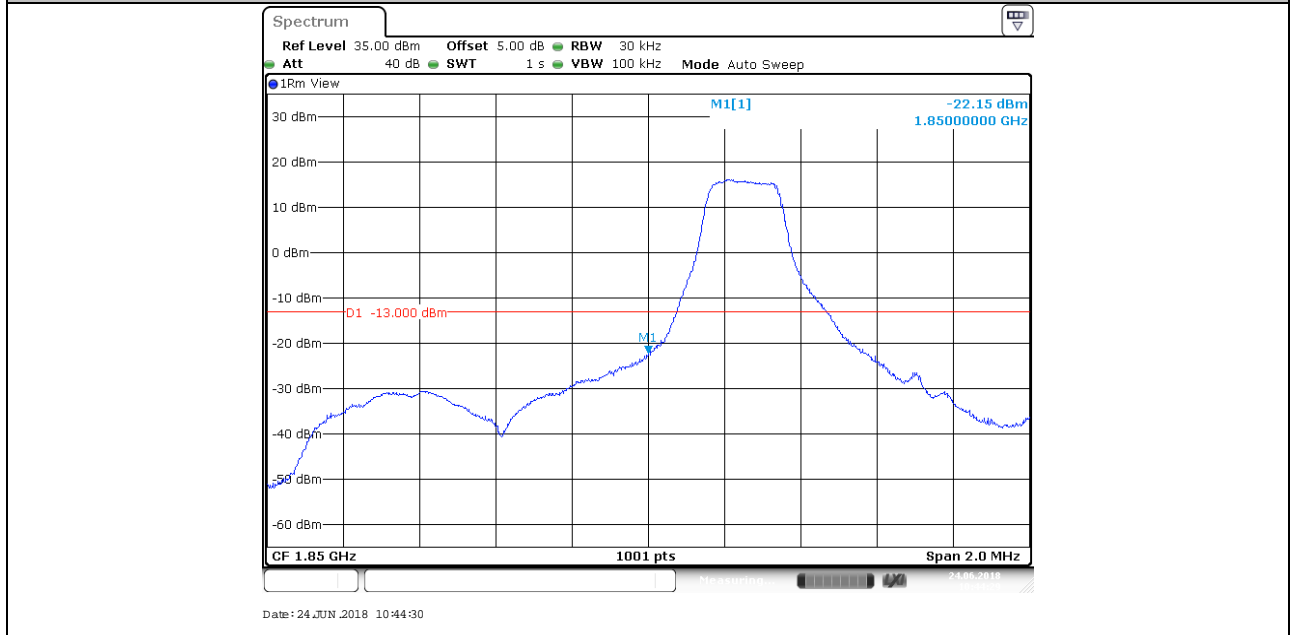
BAND 25_1.4MHz_16QAM_26047_1RB#5
