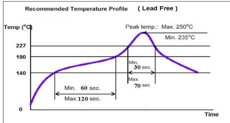
Figure 5: Reflow Profile
