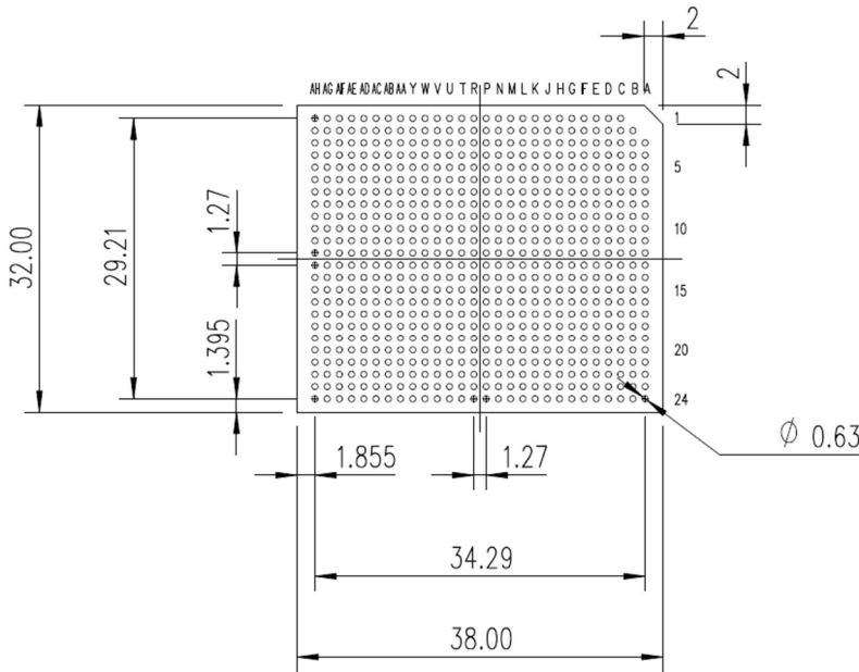
Figure 4: Land Pattern of VMC-9628
