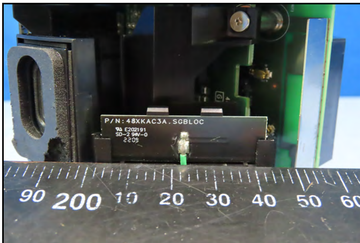
DECT1 Antenna
