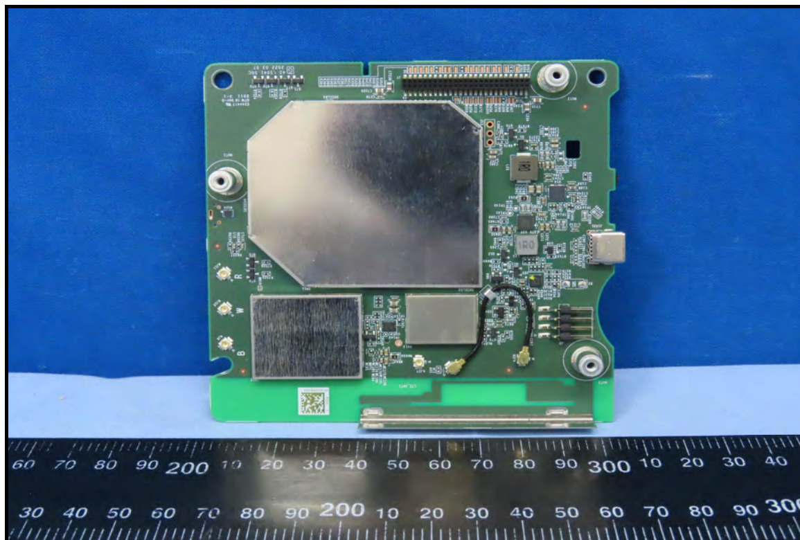
LTE Main Antenna
