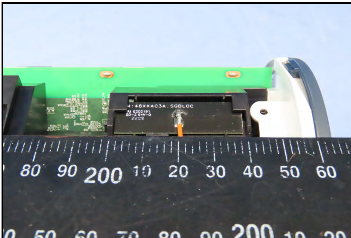
DECT2 Antenna
