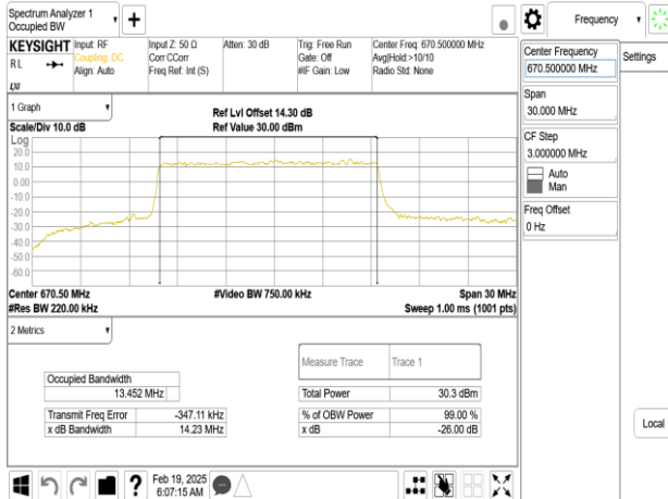
Band71_15MHz_DFT_s_OFDM_SCS15kHz_QPSK_RB75_0_CH134100
