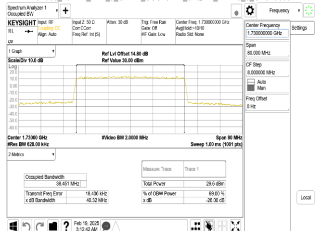
Band66_40MHz_DFT_s_OFDM_SCS15kHz_64QAM_RB216_0_CH346000
