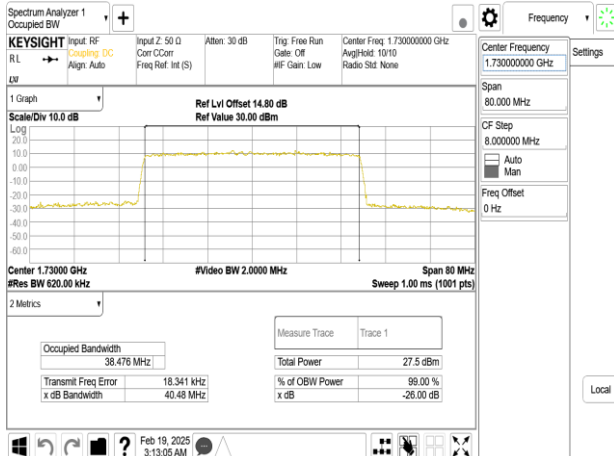
Band66_40MHz_DFT_s_OFDM_SCS15kHz_256QAM_RB216_0_CH346000
