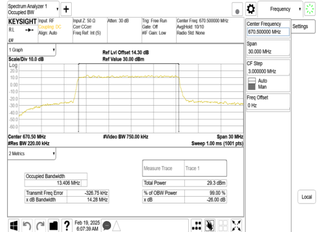
Band71_15MHz_DFT_s_OFDM_SCS15kHz_16QAM_RB75_0_CH134100
