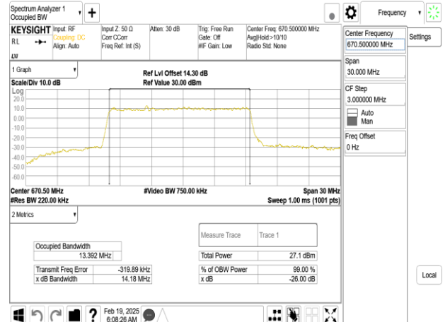
Band71_15MHz_DFT_s_OFDM_SCS15kHz_256QAM_RB75_0_CH134100
