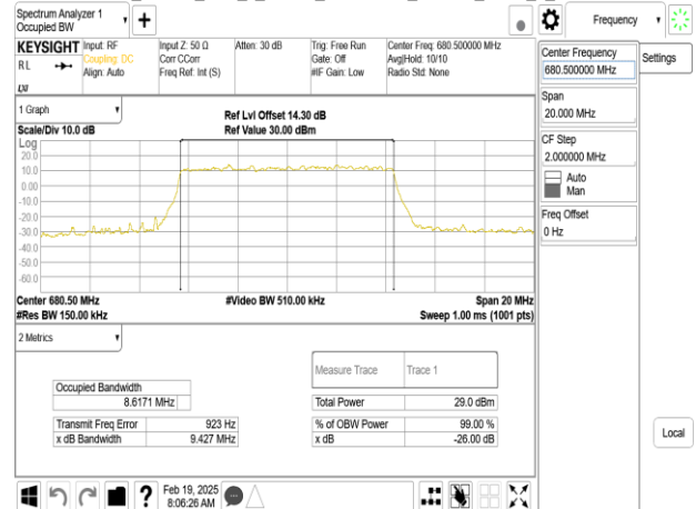
Band71_10MHz_DFT_s_OFDM_SCS30kHz_16QAM_RB24_0_CH138600
