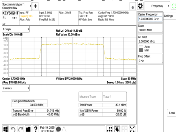
Band66_40MHz_DFT_s_OFDM_SCS15kHz_16QAM_RB216_0_CH346000
