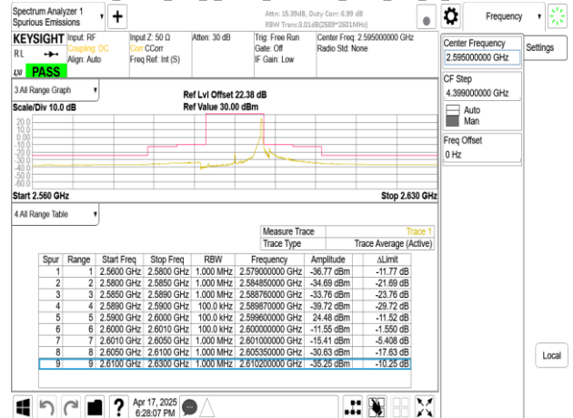
Band38_10MHz_DFT_s_OFDM_SCS15kHz_BPSK_RB50_0_CH519000
