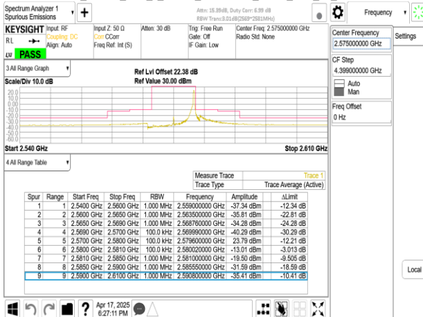
Band38_10MHz_DFT_s_OFDM_SCS15kHz_BPSK_RB50_0_CH515000
