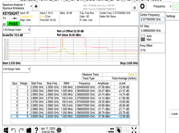
Band38_15MHz_DFT_s_OFDM_SCS15kHz_BPSK_RB1_78_CH515500
