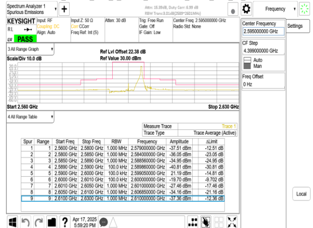
Band38_10MHz_DFT_s_OFDM_SCS30kHz_BPSK_RB24_0_CH519000
