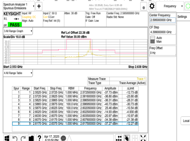
Band38_15MHz_DFT_s_OFDM_SCS15kHz_BPSK_RB75_0_CH519000
