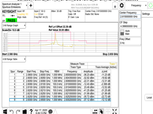
Band38_10MHz_DFT_s_OFDM_SCS15kHz_BPSK_RB1_51_CH523000
