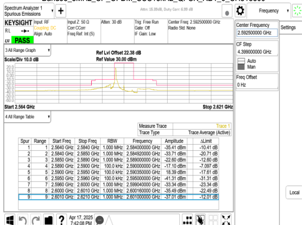
Band38_5MHz_CP_OFDM_SCS15kHz_QPSK_RB1_24_CH518500
