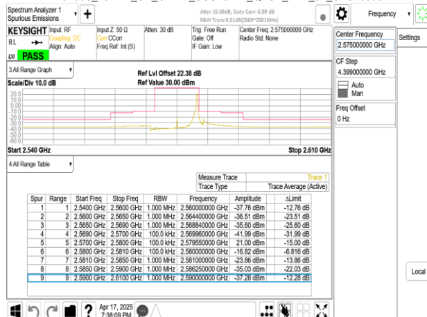
Band38_10MHz_CP_OFDM_SCS15kHz_QPSK_RB52_0_CH515000
