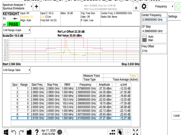
Band38_10MHz_CP_OFDM_SCS30kHz_QPSK_RB1_23_CH519000
