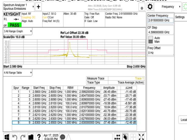
Band38_10MHz_CP_OFDM_SCS30kHz_QPSK_RB1_23_CH523000
