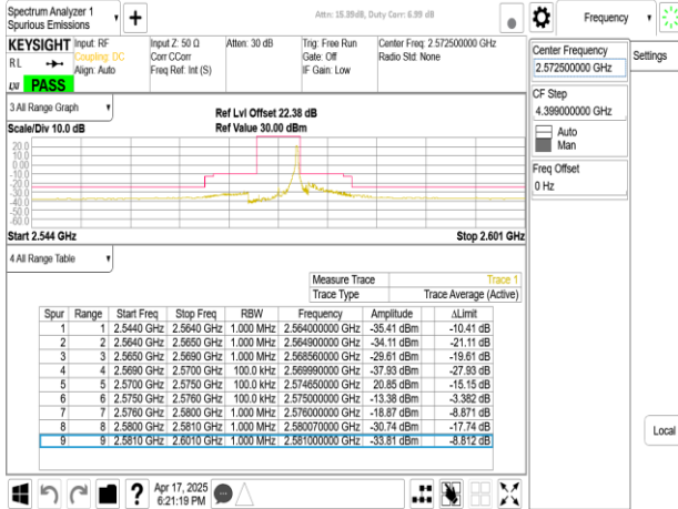
Band38_5MHz_DFT_s_OFDM_SCS15kHz_BPSK_RB25_0_CH514500
