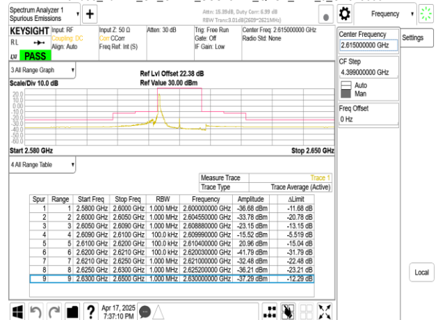
Band38_10MHz_CP_OFDM_SCS15kHz_QPSK_RB1_51_CH523000
