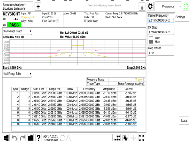
Band38_5MHz_DFT_s_OFDM_SCS15kHz_BPSK_RB25_0_CH523500
