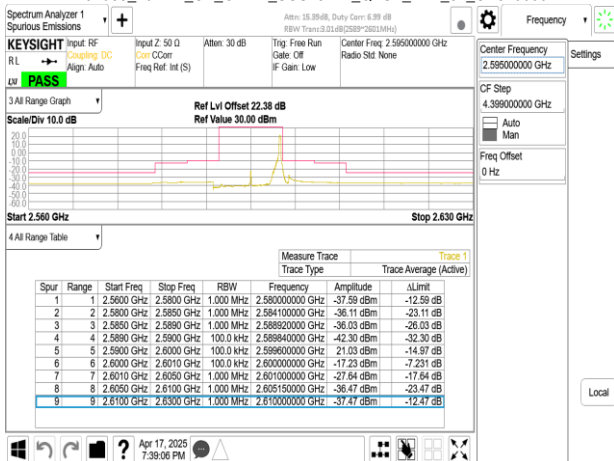
Band38_10MHz_CP_OFDM_SCS15kHz_QPSK_RB52_0_CH519000
