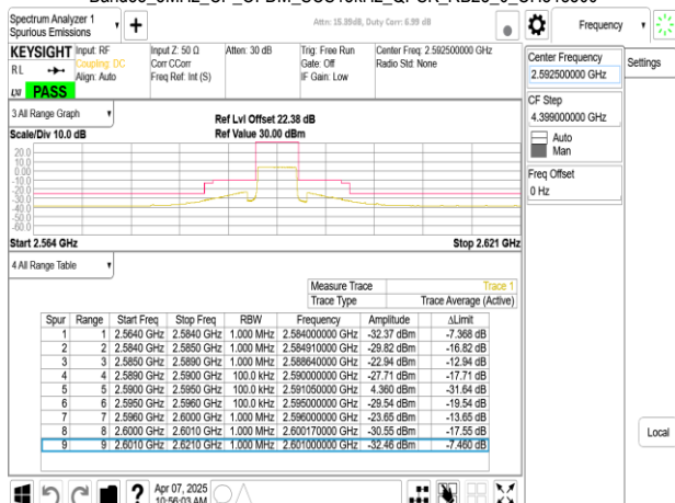
Band38_5MHz_CP_OFDM_SCS15kHz_QPSK_RB25_0_CH518500
