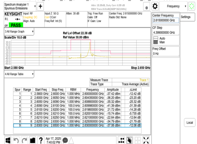
Band38_10MHz_CP_OFDM_SCS15kHz_QPSK_RB52_0_CH523000
