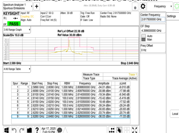
Band38_5MHz_CP_OFDM_SCS15kHz_QPSK_RB1_24_CH523500
