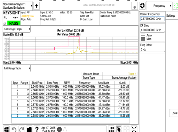
Band38_5MHz_CP_OFDM_SCS15kHz_QPSK_RB25_0_CH514500
