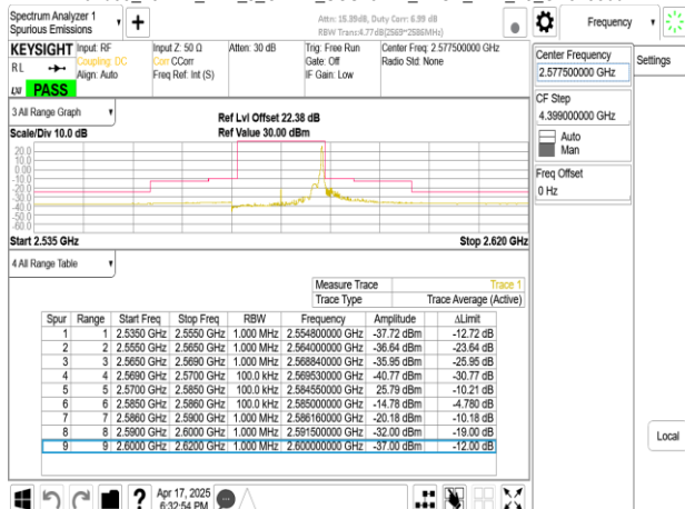
Band38_15MHz_DFT_s_OFDM_SCS15kHz_BPSK_RB75_0_CH515500
