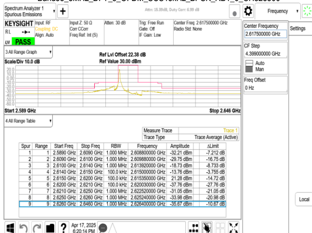
Band38_5MHz_DFT_s_OFDM_SCS15kHz_BPSK_RB1_24_CH523500
