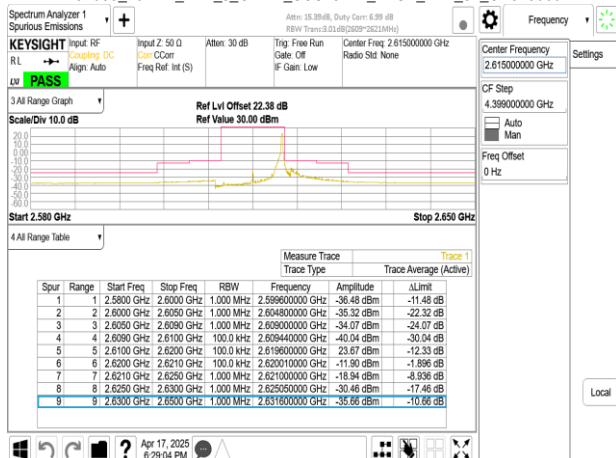
Band38_10MHz_DFT_s_OFDM_SCS15kHz_BPSK_RB50_0_CH523000
