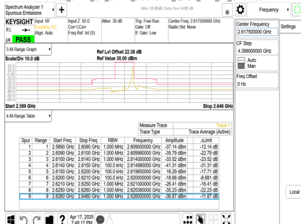
Band38_5MHz_CP_OFDM_SCS15kHz_QPSK_RB25_0_CH523500
