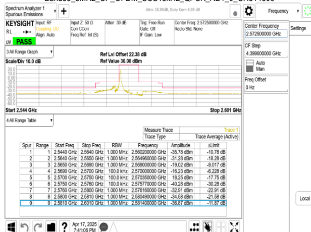
Band38_5MHz_CP_OFDM_SCS15kHz_QPSK_RB1_24_CH514500
