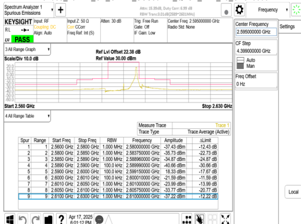
Band38_10MHz_CP_OFDM_SCS30kHz_QPSK_RB24_0_CH519000
