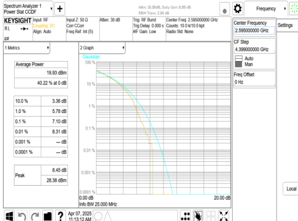
Band38_40MHz_DFT_s_OFDM_SCS15kHz_256QAM_RB216_0_CH519000
