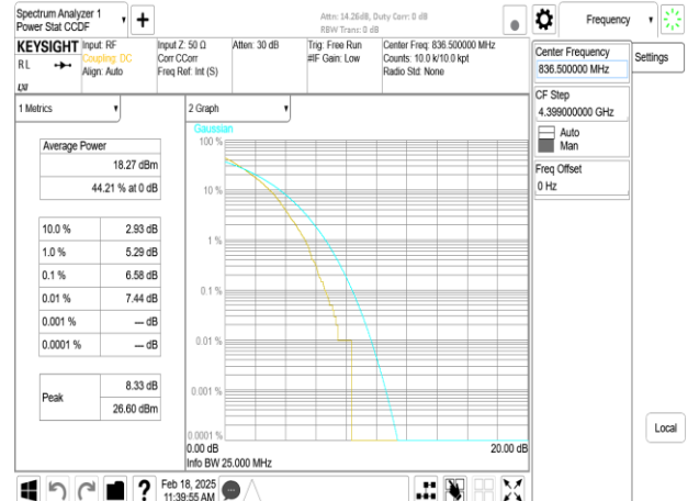
Band26_20MHz_DFT_s_OFDM_SCS15kHz_256QAM_RB100_0_CH167300
