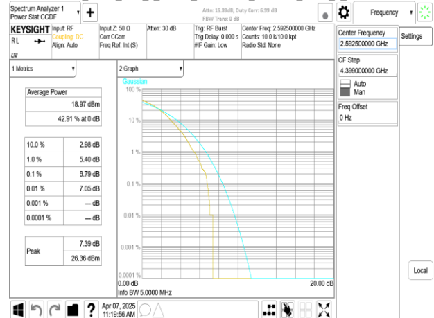
Band38_5MHz_DFT_s_OFDM_SCS15kHz_256QAM_RB25_0_CH519000
