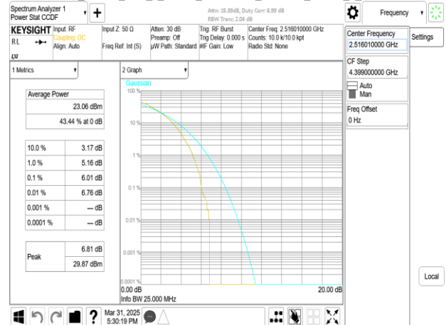
Band41_40MHz_DFT_s_OFDM_SCS30kHz_256QAM_RB100_0_CH504000
