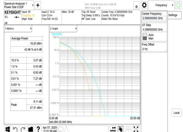
Band38_25MHz_DFT_s_OFDM_SCS30kHz_256QAM_RB64_0_CH519000
