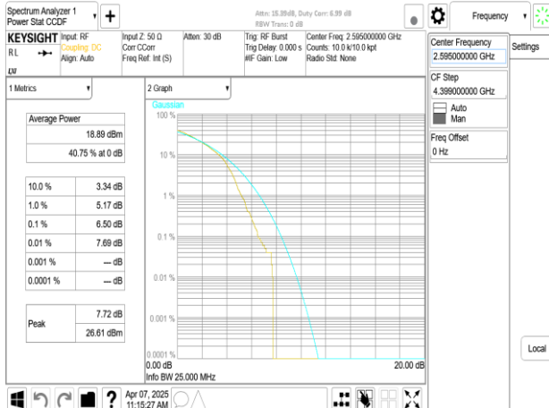
Band38_25MHz_DFT_s_OFDM_SCS15kHz_256QAM_RB128_0_CH519000
