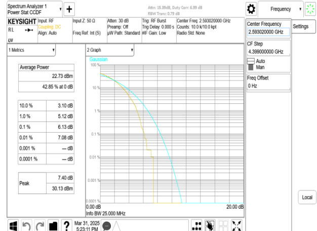
Band41_30MHz_DFT_s_OFDM_SCS15kHz_256QAM_RB160_0_CH518604
