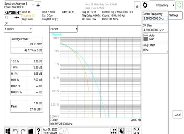
Band38_30MHz_DFT_s_OFDM_SCS30kHz_256QAM_RB75_0_CH519000
