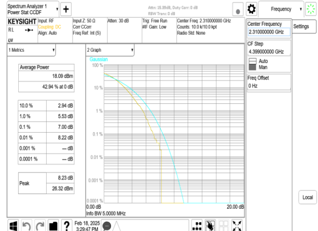
Band30_5MHz_DFT_s_OFDM_SCS15kHz_256QAM_RB25_0_CH462000
