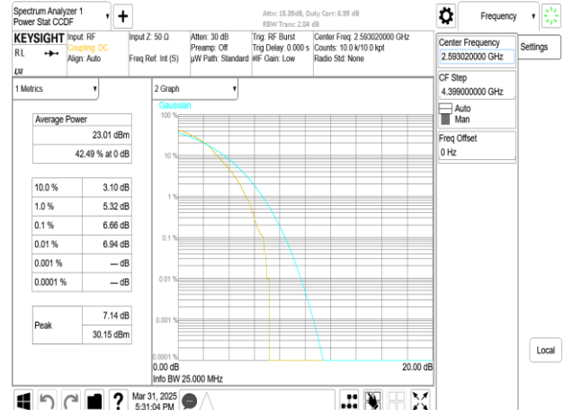
Band41_40MHz_DFT_s_OFDM_SCS30kHz_256QAM_RB100_0_CH518604
