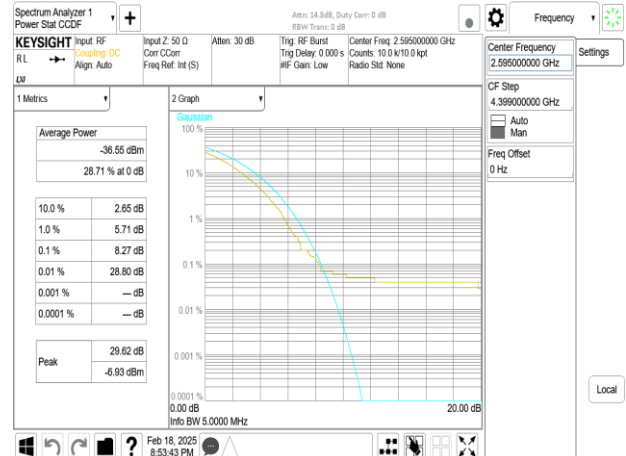
Band38_5MHz_DFT_s_OFDM_SCS15kHz_256QAM_RB25_0_CH519000
