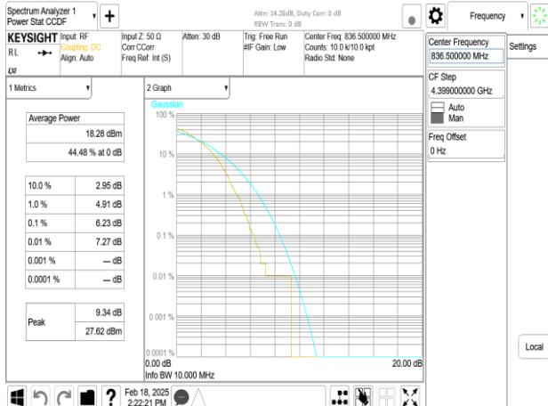
Band26_10MHz_DFT_s_OFDM_SCS30kHz_256QAM_RB24_0_CH167300
