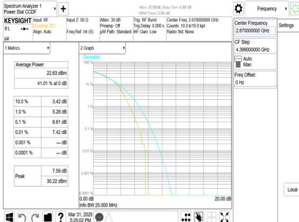
Band41_40MHz_DFT_s_OFDM_SCS15kHz_256QAM_RB216_0_CH534000
