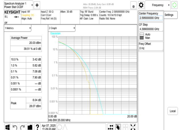
Band38_40MHz_DFT_s_OFDM_SCS30kHz_256QAM_RB100_0_CH519000
