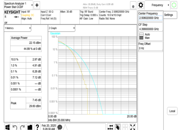
Band41_20MHz_DFT_s_OFDM_SCS30kHz_256QAM_RB50_0_CH501204
