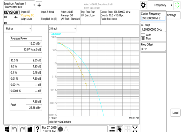
Band26_15MHz_DFT_s_OFDM_SCS15kHz_256QAM_RB75_0_CH167300
