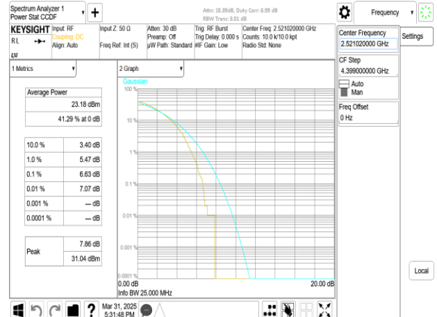
Band41_50MHz_DFT_s_OFDM_SCS30kHz_256QAM_RB128_0_CH504204
