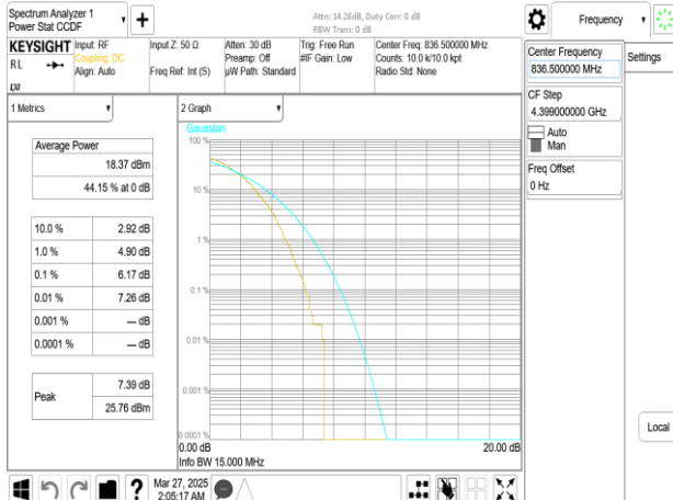
Band26_15MHz_DFT_s_OFDM_SCS30kHz_256QAM_RB36_0_CH167300
