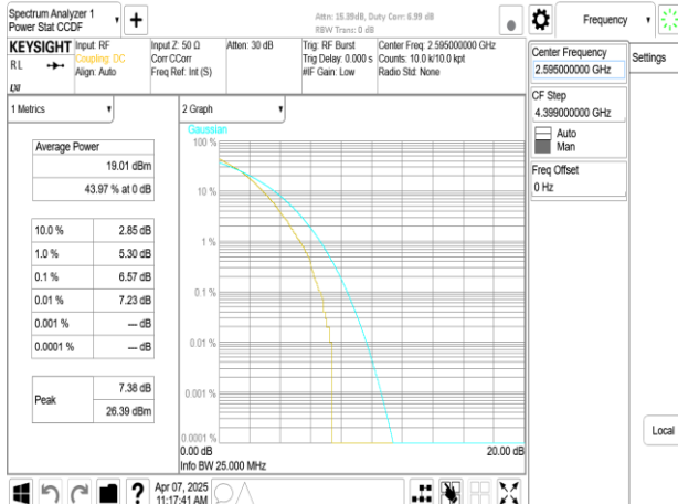
Band38_15MHz_DFT_s_OFDM_SCS15kHz_256QAM_RB75_0_CH519000
