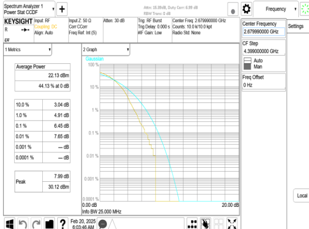
Band41_20MHz_DFT_s_OFDM_SCS30kHz_256QAM_RB50_0_CH535998
