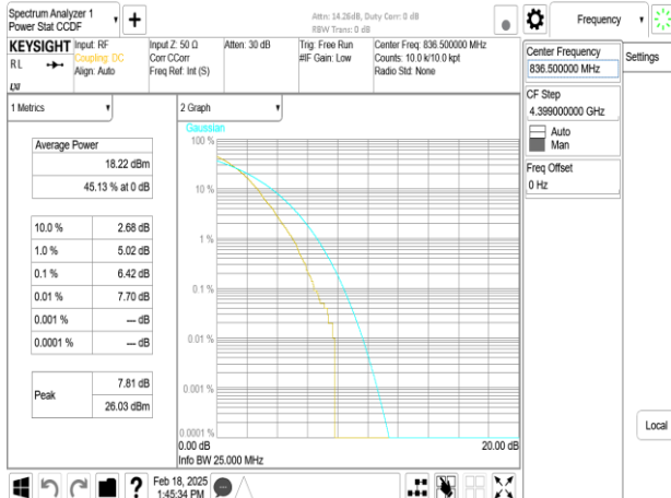
Band26_20MHz_DFT_s_OFDM_SCS30kHz_256QAM_RB50_0_CH167300
