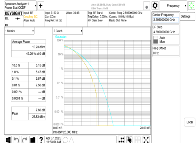
Band38_15MHz_DFT_s_OFDM_SCS30kHz_256QAM_RB36_0_CH519000
