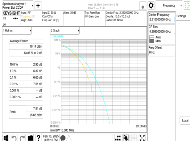
Band30_10MHz_DFT_s_OFDM_SCS30kHz_256QAM_RB24_0_CH462000
