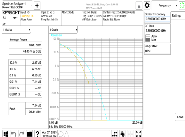
Band38_20MHz_DFT_s_OFDM_SCS15kHz_256QAM_RB100_0_CH519000
