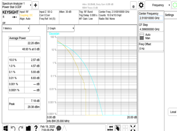
Band41_20MHz_DFT_s_OFDM_SCS15kHz_256QAM_RB100_0_CH502002
