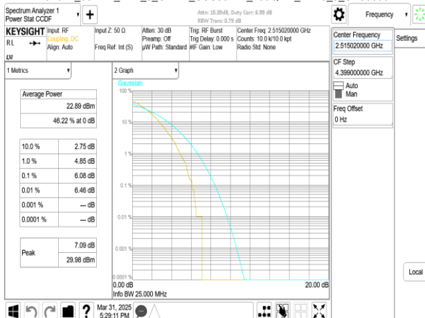
Band41_30MHz_DFT_s_OFDM_SCS30kHz_256QAM_RB75_0_CH503004
