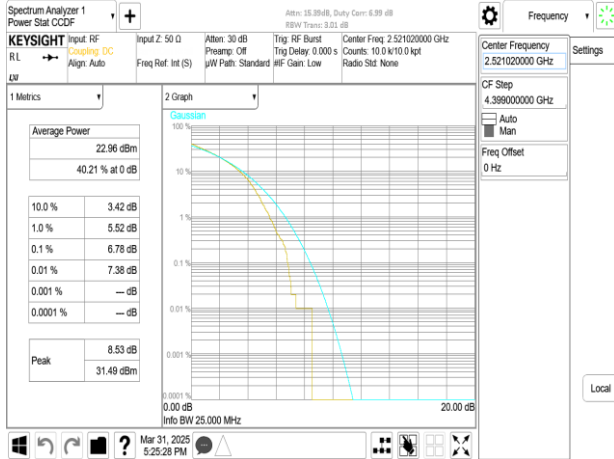
Band41_50MHz_DFT_s_OFDM_SCS15kHz_256QAM_RB270_0_CH505002
