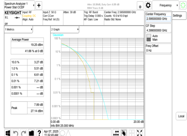
Band38_20MHz_DFT_s_OFDM_SCS30kHz_256QAM_RB50_0_CH519000
