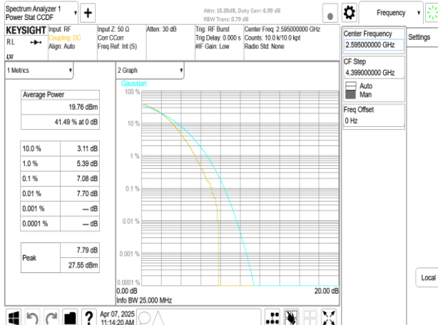
Band38_30MHz_DFT_s_OFDM_SCS15kHz_256QAM_RB160_0_CH519000
