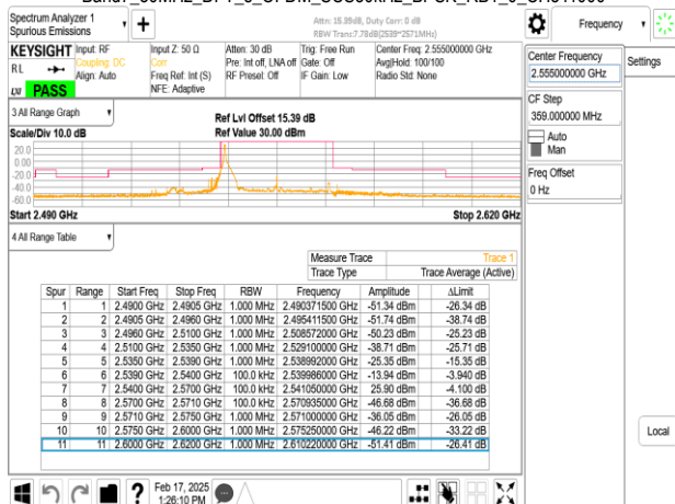
Band7_30MHz_DFT_s_OFDM_SCS30kHz_BPSK_RB1_77_CH511000
