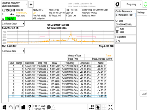
Band7_25MHz_DFT_s_OFDM_SCS30kHz_BPSK_RB64_0_CH502500
