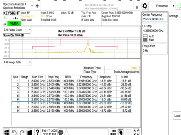
Band7_25MHz_CP_OFDM_SCS30kHz_QPSK_RB65_0_CH511500
