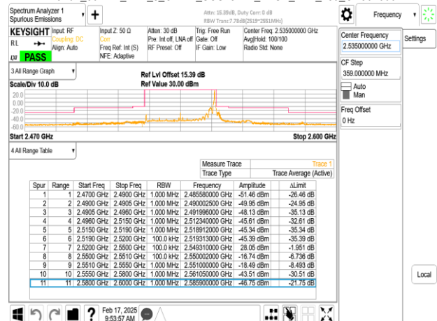
Band7_30MHz_DFT_s_OFDM_SCS15kHz_BPSK_RB1_159_CH507000
