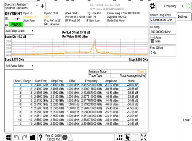
Band7_30MHz_DFT_s_OFDM_SCS30kHz_BPSK_RB75_0_CH507000
