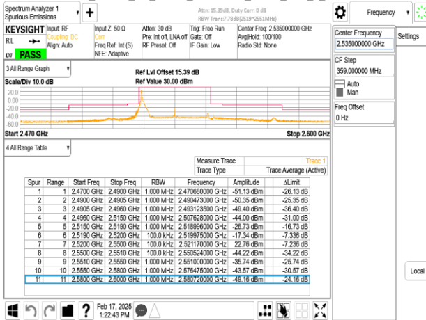
Band7_30MHz_CP_OFDM_SCS30kHz_QPSK_RB1_77_CH507000
