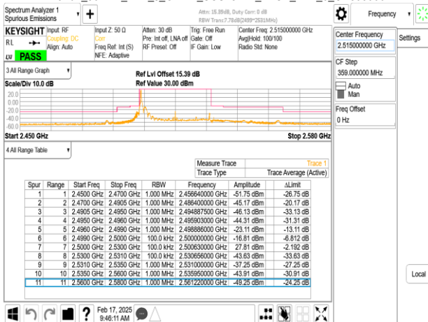
Band7_30MHz_DFT_s_OFDM_SCS15kHz_BPSK_RB1_159_CH503000
