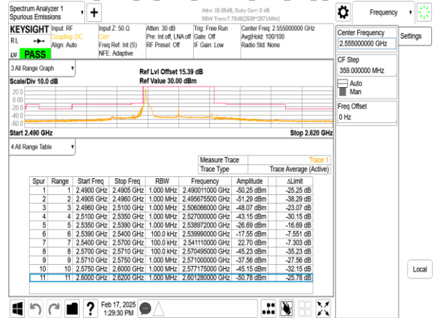
Band7_30MHz_CP_OFDM_SCS30kHz_QPSK_RB1_77_CH511000
