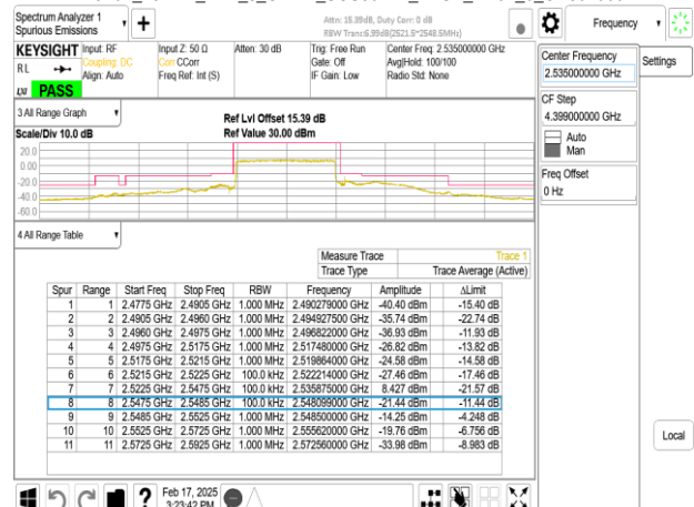
Band7_25MHz_DFT_s_OFDM_SCS30kHz_BPSK_RB64_0_CH507000
