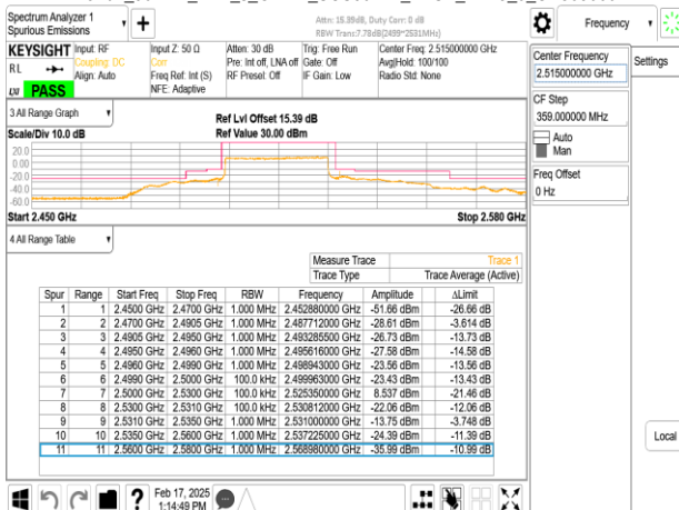
Band7_30MHz_DFT_s_OFDM_SCS30kHz_BPSK_RB75_0_CH503000
