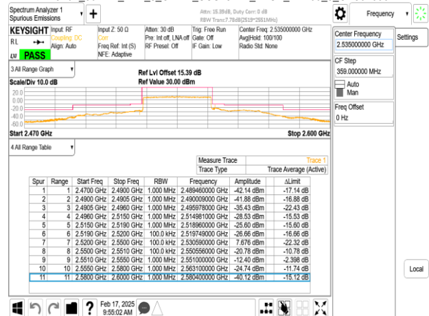
Band7_30MHz_DFT_s_OFDM_SCS15kHz_BPSK_RB1_0_CH507000
