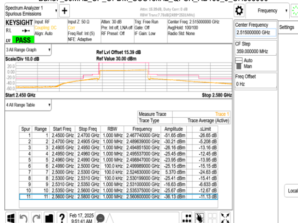
Band7_30MHz_CP_OFDM_SCS15kHz_QPSK_RB1_0_CH503000
