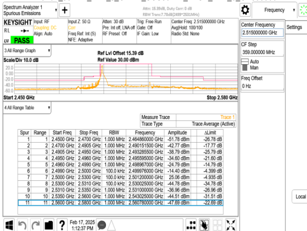
Band7_30MHz_DFT_s_OFDM_SCS30kHz_BPSK_RB1_77_CH503000
