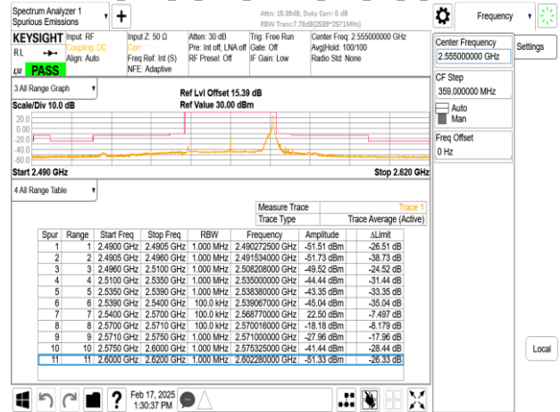
Band7_30MHz_CP_OFDM_SCS30kHz_QPSK_RB78_0_CH511000
