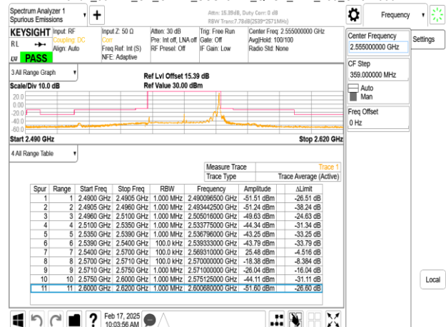
Band7_30MHz_CP_OFDM_SCS15kHz_QPSK_RB1_159_CH511000
