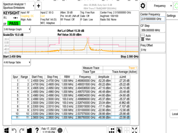
Band7_30MHz_CP_OFDM_SCS30kHz_QPSK_RB78_0_CH503000
