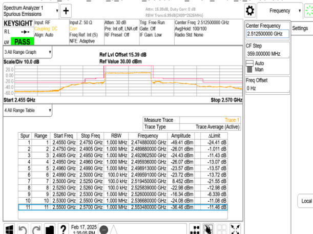
Band7_25MHz_DFT_s_OFDM_SCS30kHz_BPSK_RB64_0_CH502500
