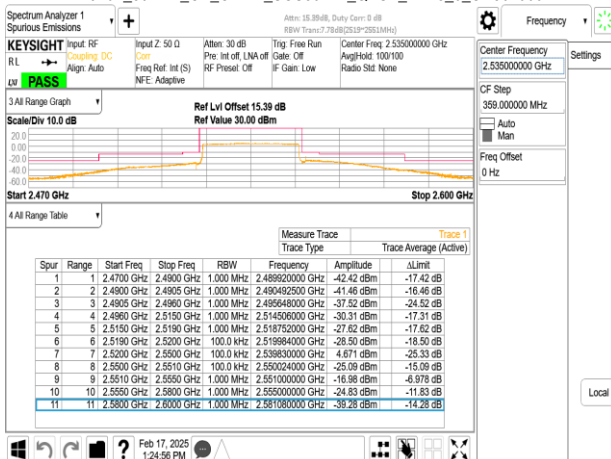
Band7_30MHz_CP_OFDM_SCS30kHz_QPSK_RB78_0_CH507000
