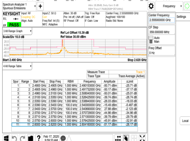
Band7_30MHz_DFT_s_OFDM_SCS15kHz_BPSK_RB1_159_CH511000
