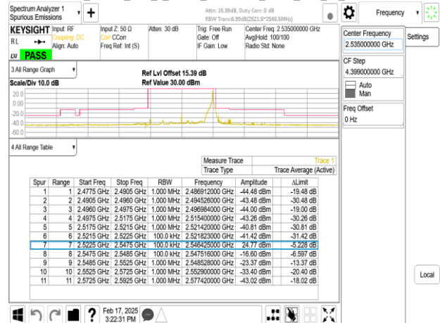
Band7_25MHz_DFT_s_OFDM_SCS30kHz_BPSK_RB64_0_CH507000
