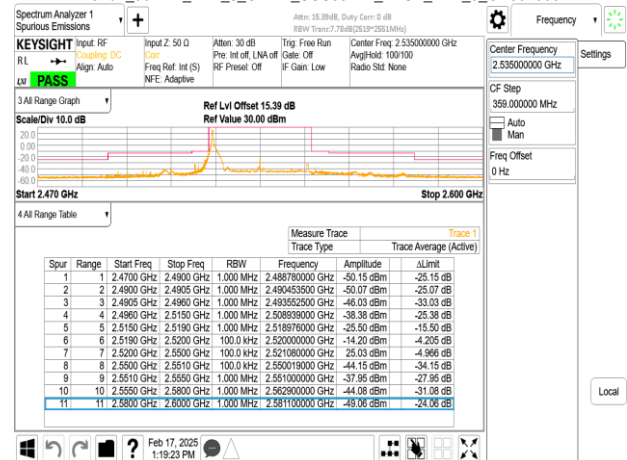
Band7_30MHz_DFT_s_OFDM_SCS30kHz_BPSK_RB1_77_CH507000
