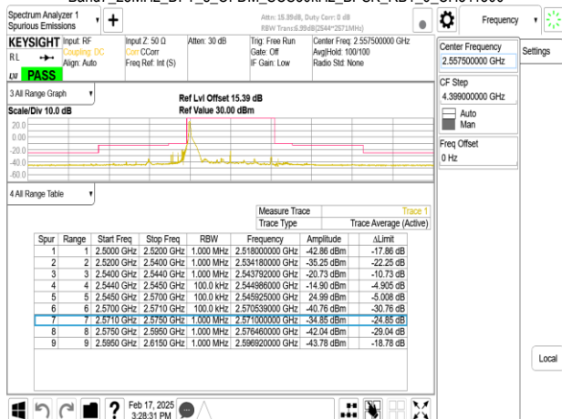
Band7_25MHz_DFT_s_OFDM_SCS30kHz_BPSK_RB1_64_CH511500
