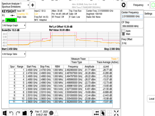
Band7_30MHz_DFT_s_OFDM_SCS15kHz_BPSK_RB1_0_CH503000
