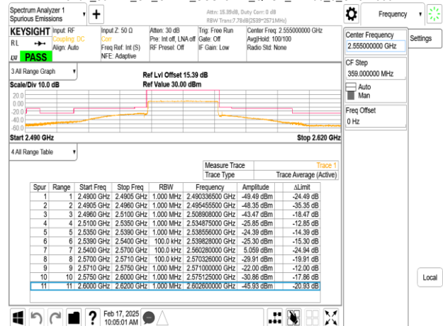
Band7_30MHz_CP_OFDM_SCS15kHz_QPSK_RB1_0_CH511000
