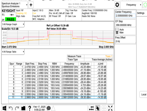
Band7_30MHz_CP_OFDM_SCS15kHz_QPSK_RB1_0_CH507000
