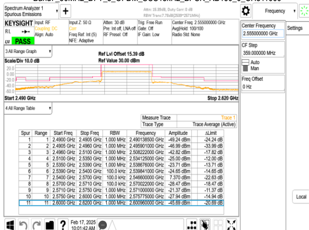
Band7_30MHz_DFT_s_OFDM_SCS15kHz_BPSK_RB1_0_CH511000
