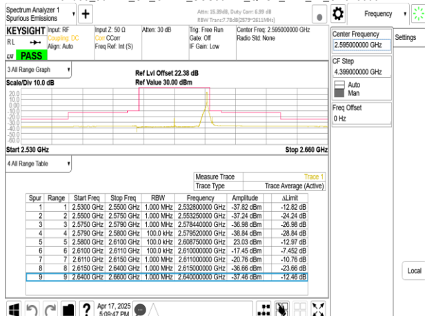
Band38_30MHz_CP_OFDM_SCS30kHz_QPSK_RB78_0_CH519000
