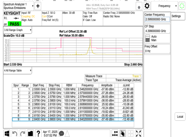
Band38_30MHz_DFT_s_OFDM_SCS30kHz_BPSK_RB75_0_CH519000
