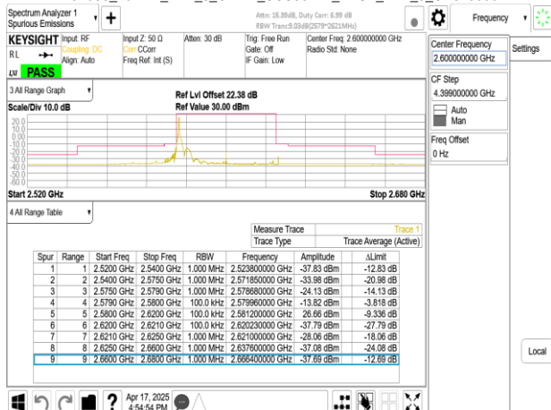
Band38_40MHz_DFT_s_OFDM_SCS30kHz_BPSK_RB1_105_CH520000
