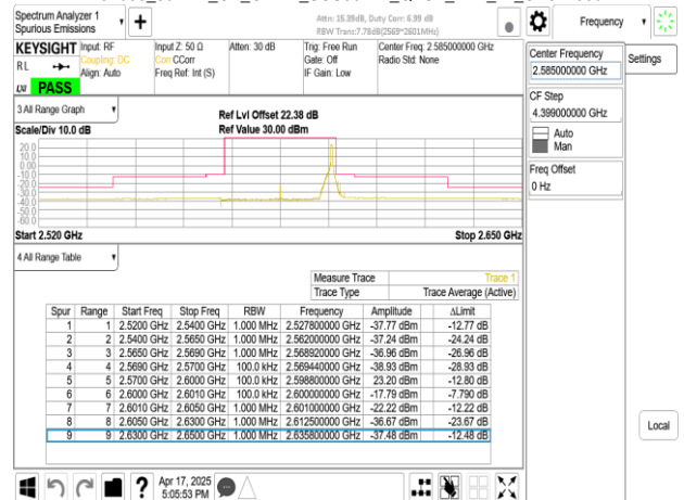
Band38_30MHz_CP_OFDM_SCS30kHz_QPSK_RB78_0_CH517000
