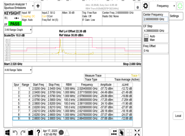
Band38_40MHz_CP_OFDM_SCS30kHz_QPSK_RB1_105_CH520000
