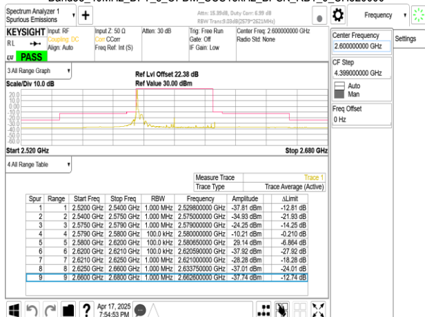
Band38_40MHz_DFT_s_OFDM_SCS15kHz_BPSK_RB1_215_CH520000
