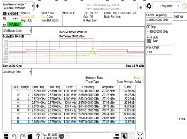
Band38_40MHz_CP_OFDM_SCS15kHz_QPSK_RB216_0_CH519000
