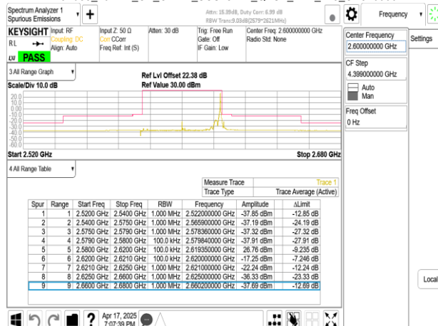
Band38_40MHz_CP_OFDM_SCS15kHz_QPSK_RB216_0_CH520000
