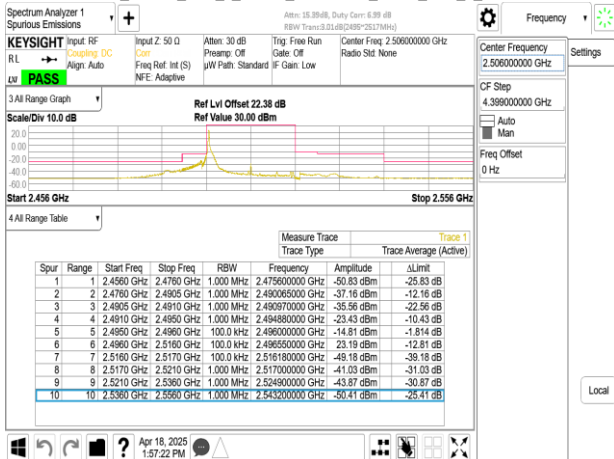
Band41_20MHz_DFT_s_OFDM_SCS15kHz_BPSK_RB1_105_CH501204
