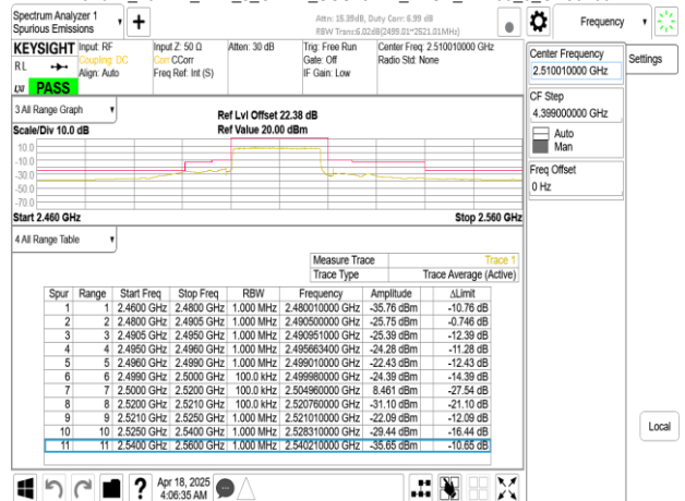
Band41_20MHz_DFT_s_OFDM_SCS15kHz_BPSK_RB1_0_CH502002
