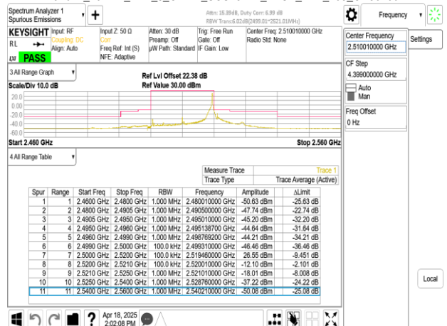
Band41_20MHz_DFT_s_OFDM_SCS15kHz_BPSK_RB1_105_CH502002
