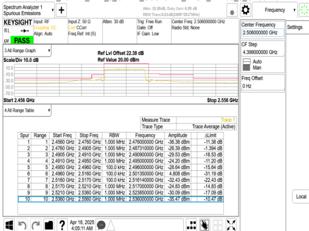
Band41_20MHz_DFT_s_OFDM_SCS15kHz_BPSK_RB1_0_CH501204
