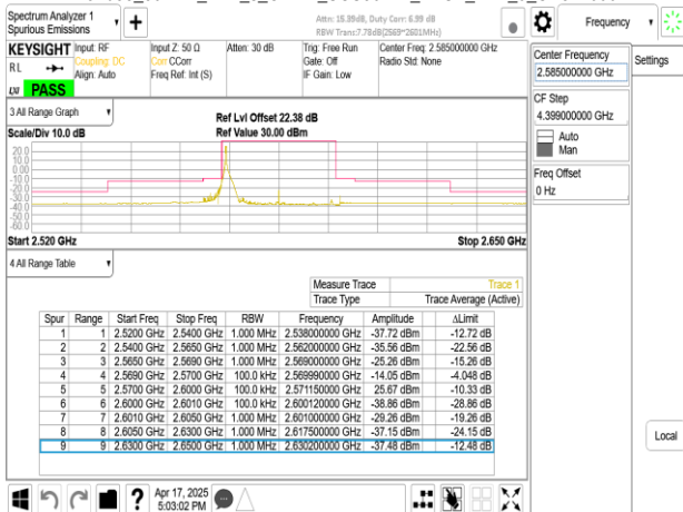
Band38_30MHz_DFT_s_OFDM_SCS30kHz_BPSK_RB1_77_CH517000
