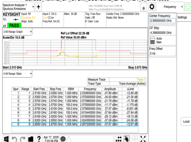
Band38_40MHz_CP_OFDM_SCS15kHz_QPSK_RB1_215_CH519000
