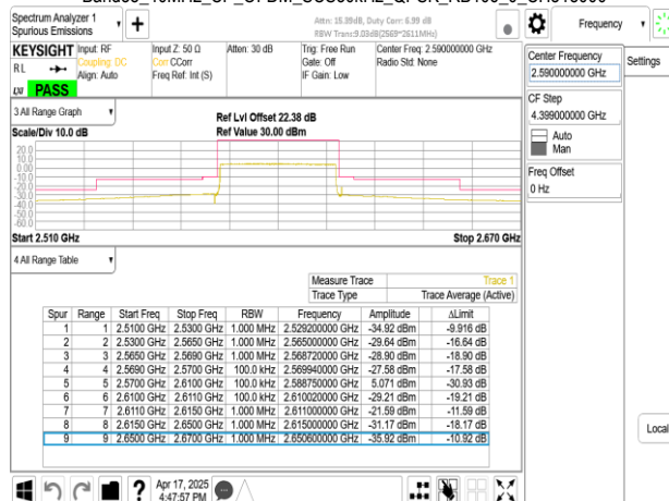
Band38_40MHz_CP_OFDM_SCS30kHz_QPSK_RB1_0_CH518000
