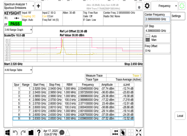
Band38_30MHz_CP_OFDM_SCS30kHz_QPSK_RB1_77_CH517000
