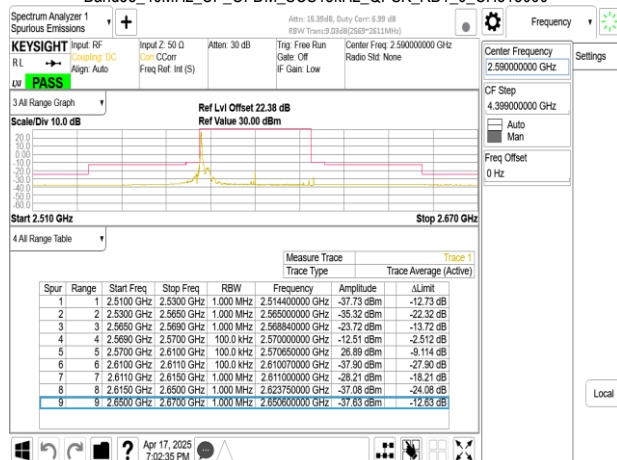
Band38_40MHz_CP_OFDM_SCS15kHz_QPSK_RB1_215_CH518000
