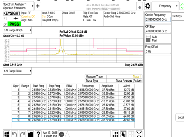
Band38_40MHz_DFT_s_OFDM_SCS30kHz_BPSK_RB1_105_CH519000
