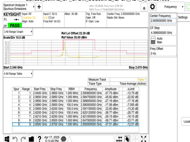
Band38_30MHz_CP_OFDM_SCS30kHz_QPSK_RB1_77_CH521000
