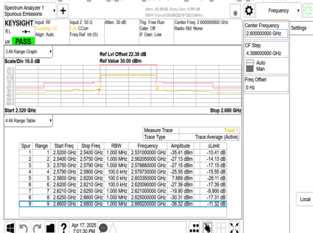
Band38_40MHz_DFT_s_OFDM_SCS15kHz_BPSK_RB216_0_CH520000
