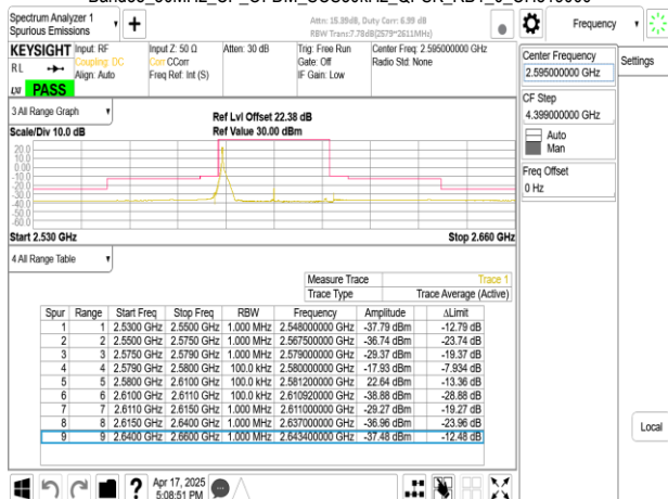
Band38_30MHz_CP_OFDM_SCS30kHz_QPSK_RB1_77_CH519000
