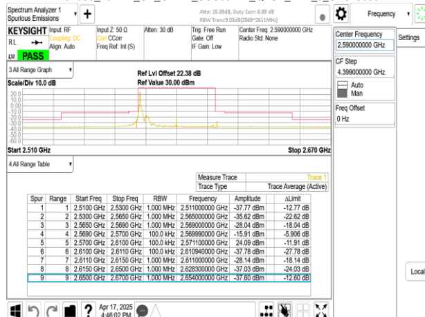
Band38_40MHz_CP_OFDM_SCS30kHz_QPSK_RB1_105_CH518000
