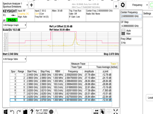
Band38_30MHz_CP_OFDM_SCS30kHz_QPSK_RB78_0_CH521000
