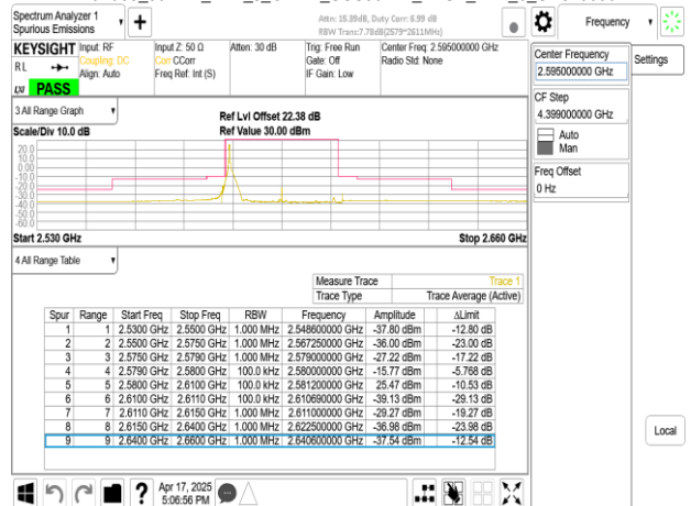
Band38_30MHz_DFT_s_OFDM_SCS30kHz_BPSK_RB1_77_CH519000
