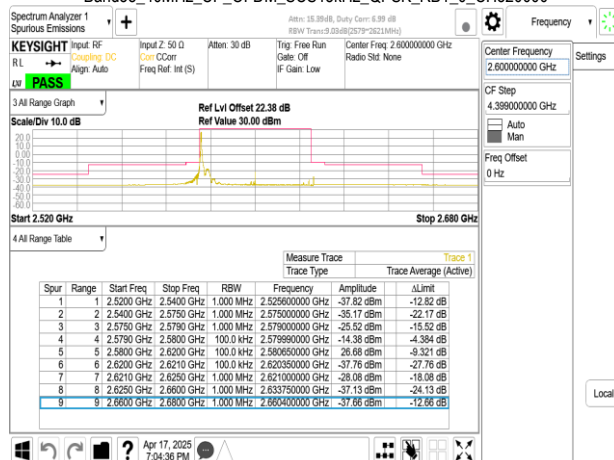
Band38_40MHz_CP_OFDM_SCS15kHz_QPSK_RB1_215_CH520000
