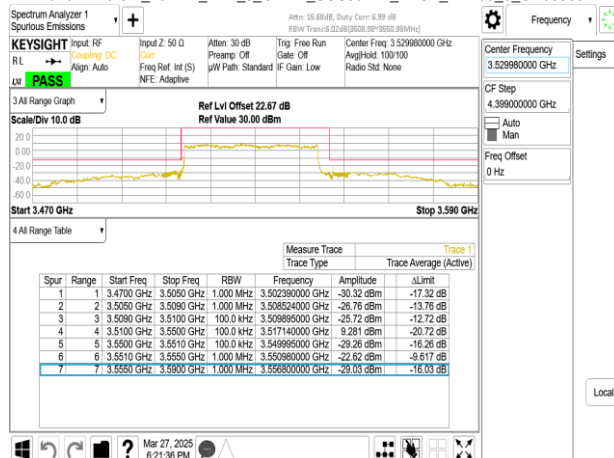
Band77-Part27_40MHz_DFT_s_OFDM_SCS30kHz_BPSK_RB1_0_CH635332
