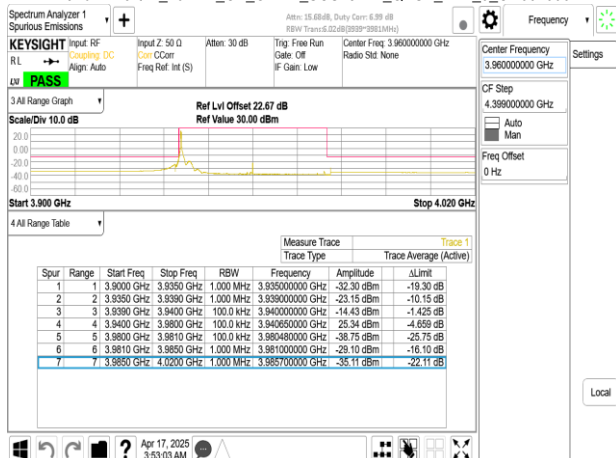
Band77-Part27_40MHz_CP_OFDM_SCS15kHz_QPSK_RB1_215_CH664000
