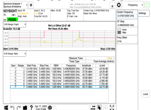
Band77-Part27_40MHz_CP_OFDM_SCS15kHz_QPSK_RB1_215_CH631334
