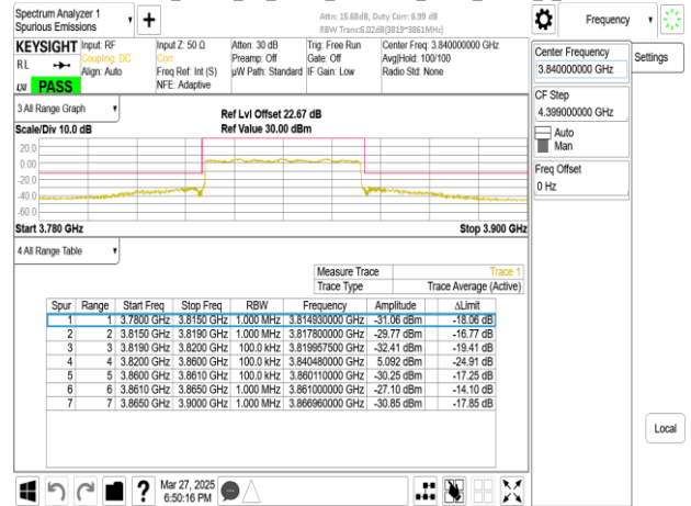
Band77-Part27_40MHz_CP_OFDM_SCS30kHz_QPSK_RB1_0_CH656000
