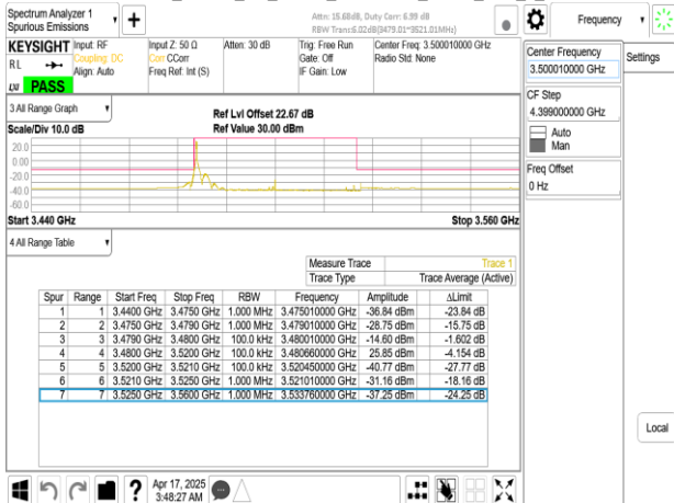
Band77-Part27_40MHz_CP_OFDM_SCS15kHz_QPSK_RB1_215_CH633334
