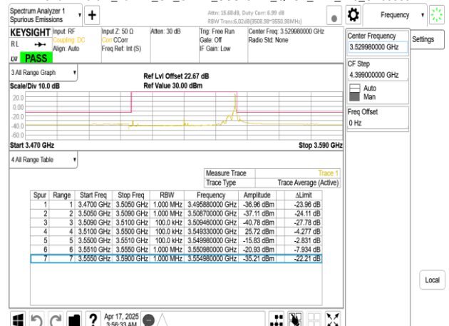
Band77-Part27_40MHz_CP_OFDM_SCS15kHz_QPSK_RB1_215_CH635332
