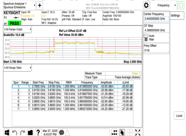
Band77-Part27_40MHz_DFT_s_OFDM_SCS30kHz_BPSK_RB1_0_CH656000
