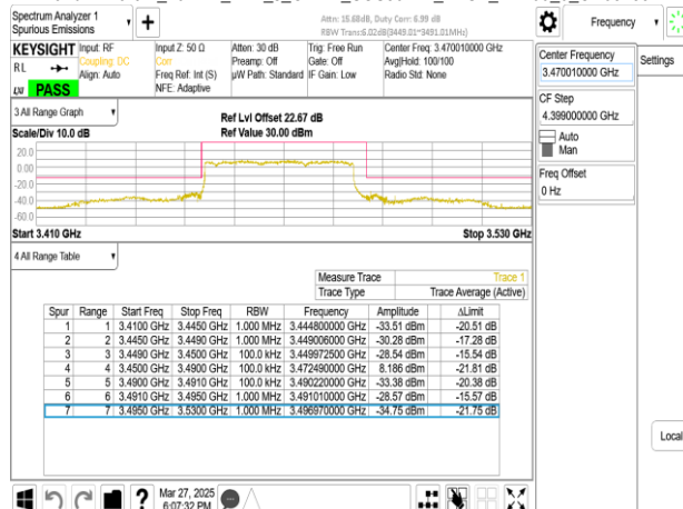
Band77-Part27_40MHz_DFT_s_OFDM_SCS30kHz_BPSK_RB1_0_CH631334
