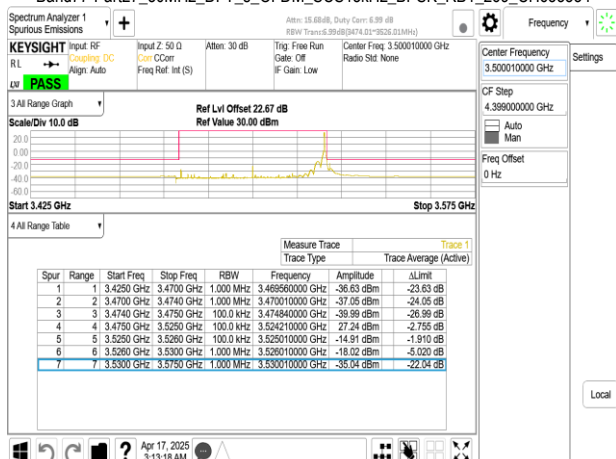
Band77-Part27_50MHz_DFT_s_OFDM_SCS15kHz_BPSK_RB1_269_CH633334
