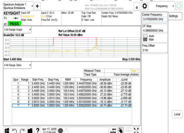
Band77-Part27_50MHz_DFT_s_OFDM_SCS15kHz_BPSK_RB1_269_CH631668
