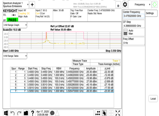
Band77-Part27_50MHz_DFT_s_OFDM_SCS15kHz_BPSK_RB1_269_CH631668
