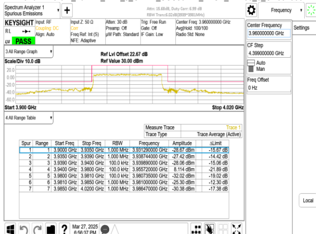
Band77-Part27_40MHz_DFT_s_OFDM_SCS30kHz_BPSK_RB1_0_CH664000
