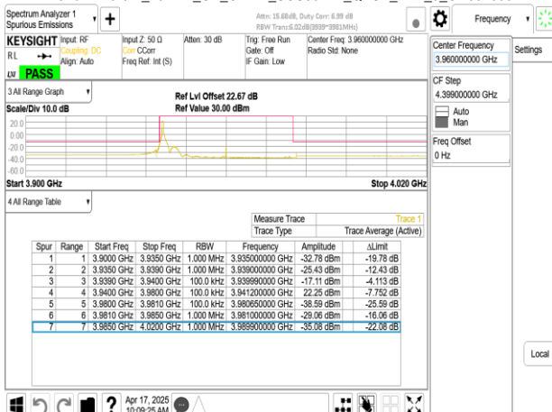
Band77-Part27_40MHz_CP_OFDM_SCS30kHz_QPSK_RB1_0_CH664000
