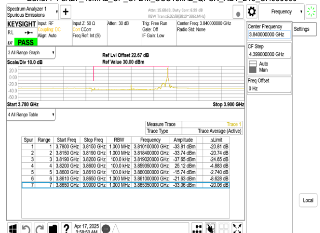
Band77-Part27_40MHz_CP_OFDM_SCS15kHz_QPSK_RB1_215_CH656000
