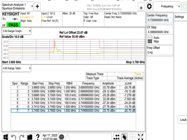
Band77-Part27_40MHz_CP_OFDM_SCS30kHz_QPSK_RB1_0_CH648000
