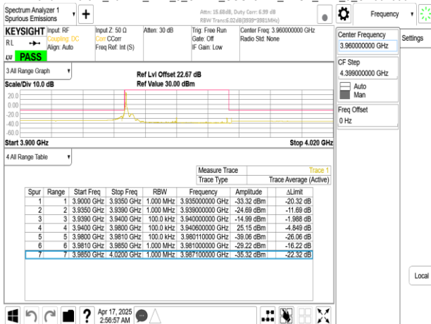
Band77-Part27_40MHz_DFT_s_OFDM_SCS15kHz_BPSK_RB1_215_CH664000
