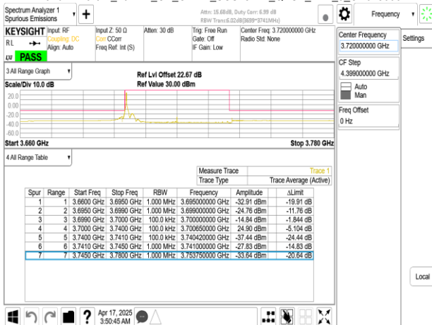
Band77-Part27_40MHz_CP_OFDM_SCS15kHz_QPSK_RB1_215_CH648000
