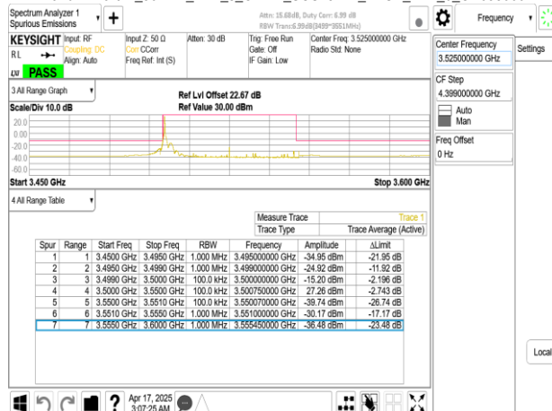
Band77-Part27_50MHz_DFT_s_OFDM_SCS15kHz_BPSK_RB1_269_CH635000
