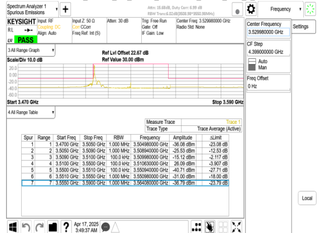
Band77-Part27_40MHz_CP_OFDM_SCS15kHz_QPSK_RB1_215_CH635332
