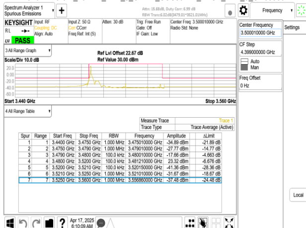
Band77-Part27_40MHz_DFT_s_OFDM_SCS30kHz_BPSK_RB1_0_CH633334
