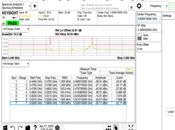
Band77-Part27_40MHz_CP_OFDM_SCS15kHz_QPSK_RB1_215_CH633334
