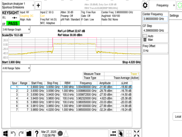
Band77-Part27_40MHz_CP_OFDM_SCS30kHz_QPSK_RB1_0_CH664000
