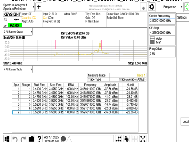
Band77-Part27_40MHz_DFT_s_OFDM_SCS30kHz_BPSK_RB100_0_CH635332
