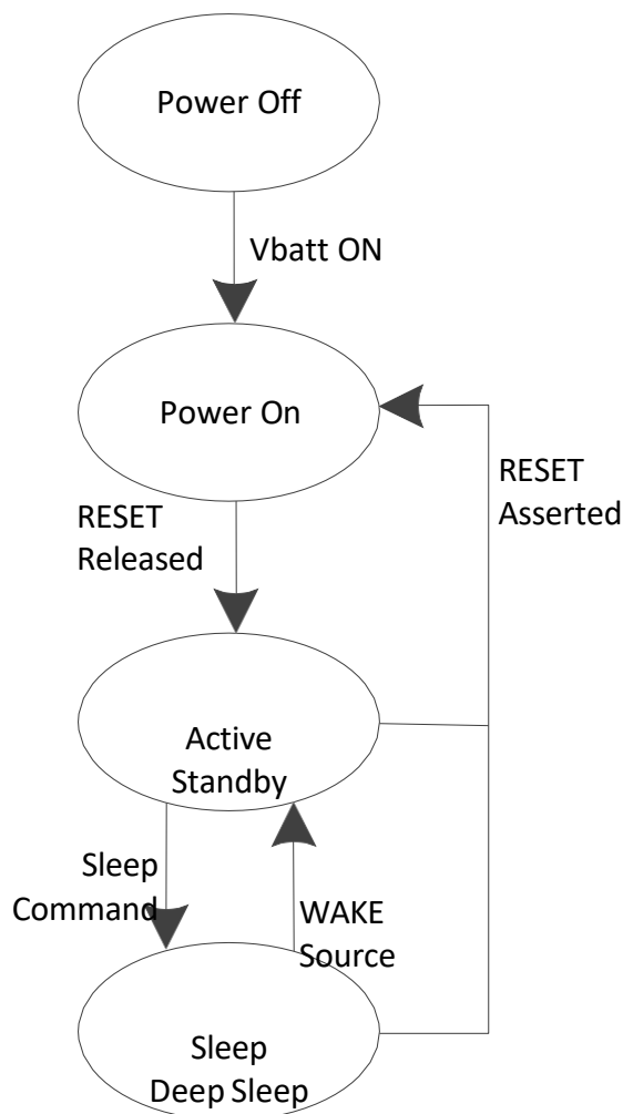
Figure 9. Electrical States and Transitions
