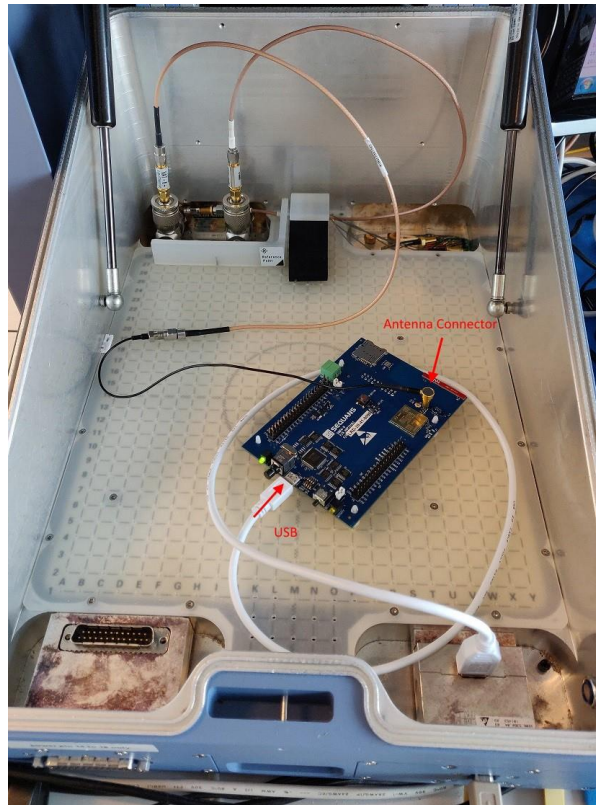
Figure 26. Shield Box Cavity View
