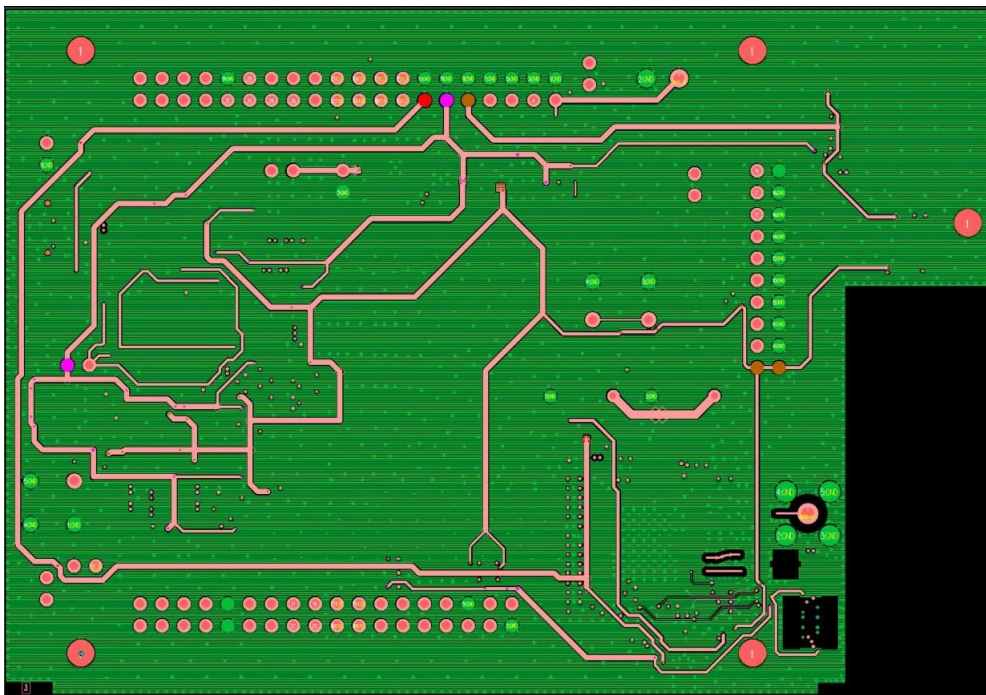
Figure 19. Layer 3 View
