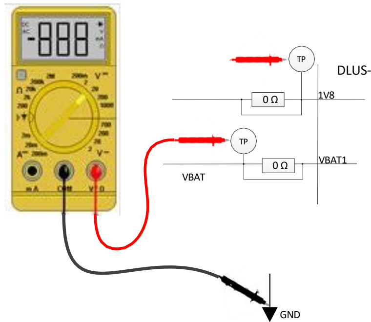
Figure 30. Measuring Voltage Value (DLUS-WI01-NA)
