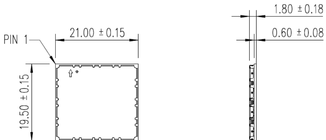
Figure 33. Module PCB View
