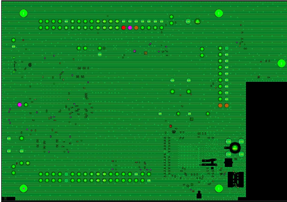
Figure 18. Layer 2 View
