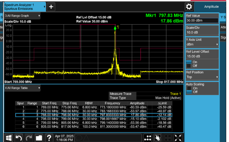
FULL CH 23378 (797.8 MHz)
