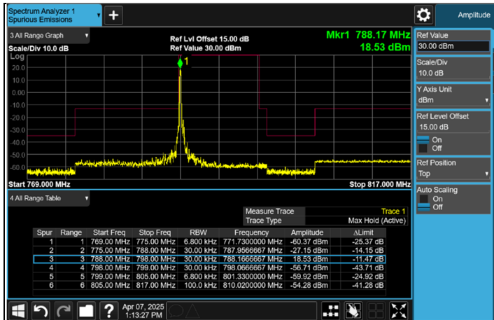
FULL CH 23282 (788.2 MHz)
