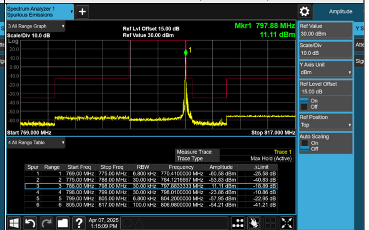
1RB CH 23378 (797.8 MHz)
