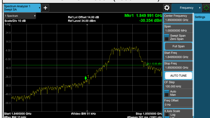
FULL CH 18607 (1850.7 MHz)
